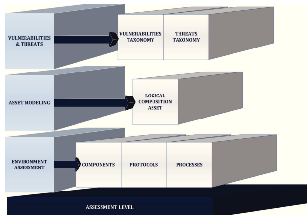
Figure 3.2: SL1-Assessment
