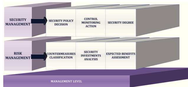
Figure 3.4: SL3-Management
