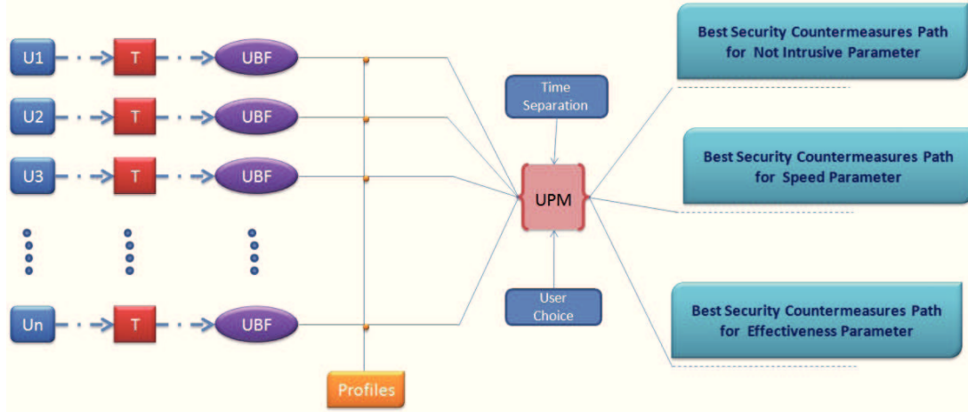
Figure 4.3: User-Profile Framework
