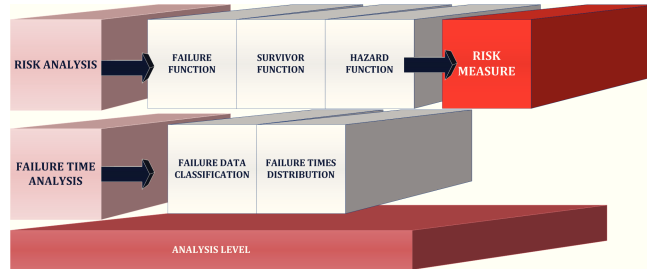
Figure 3.3: SL2-Analysis
