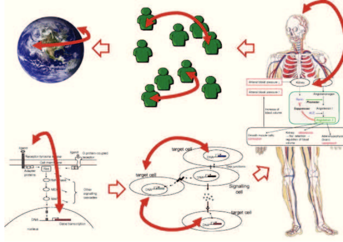
Figure 2.9: Bio-Inspired Approach
