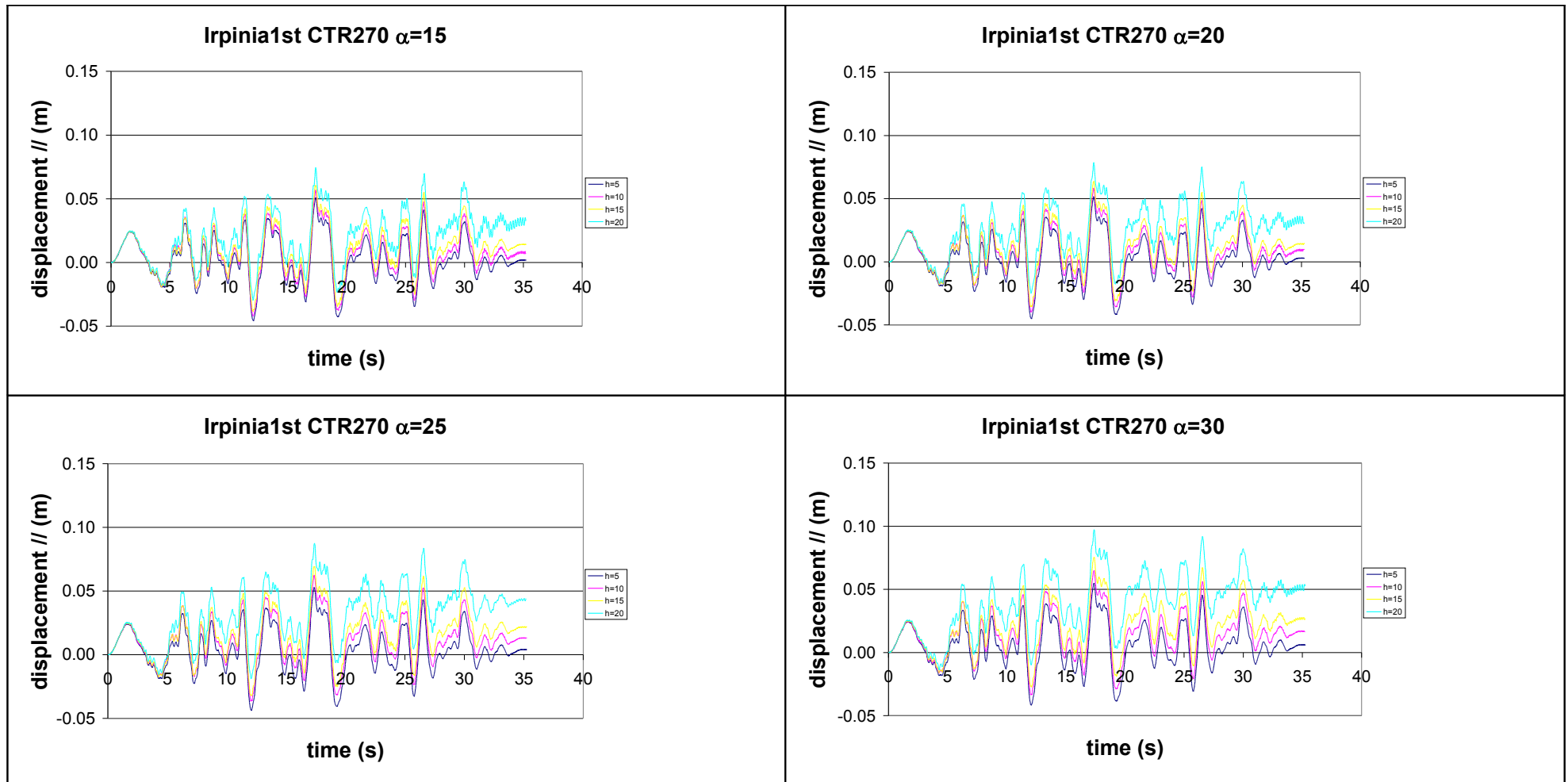
Figure 5.7. Permanent horizontal displacement, accelerometer CTR270, soil type A, Toyoura sand.
