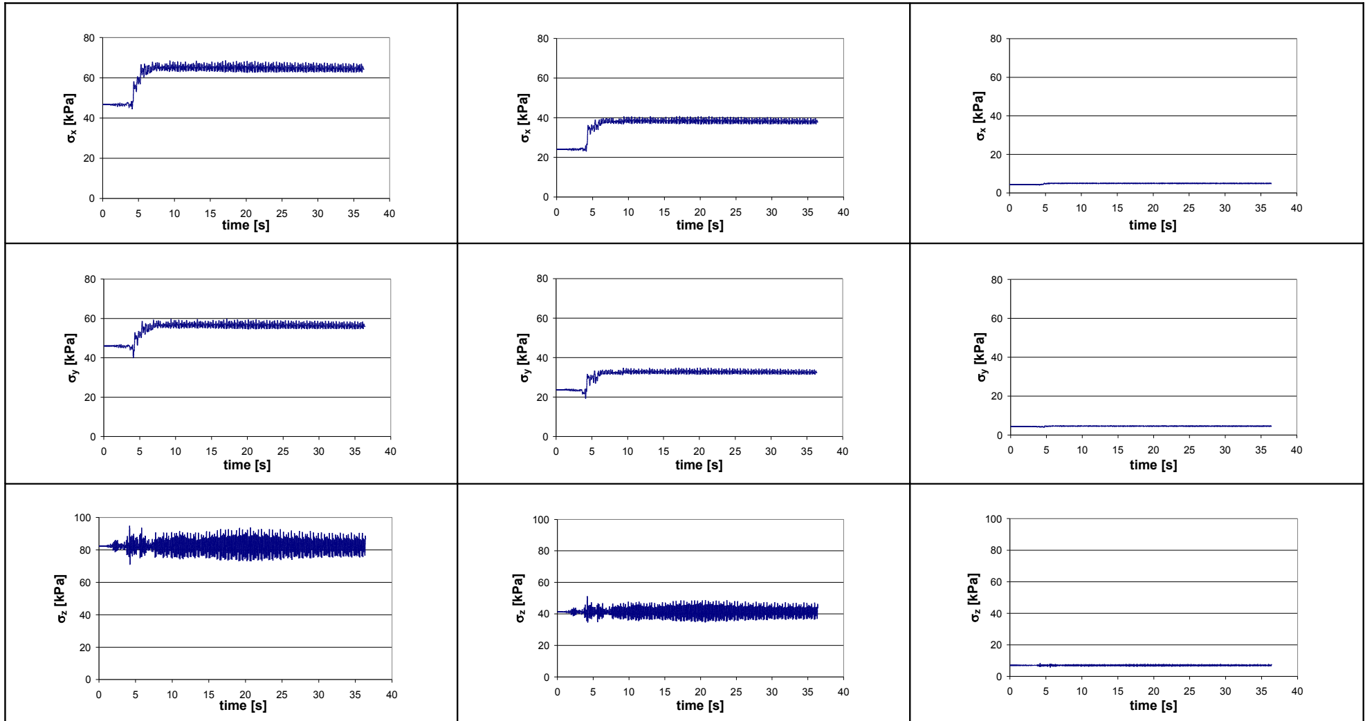
Figure 4.2 (b). Stress in x, y and z direction (base, middle and top of the layer), Hostun sand.
