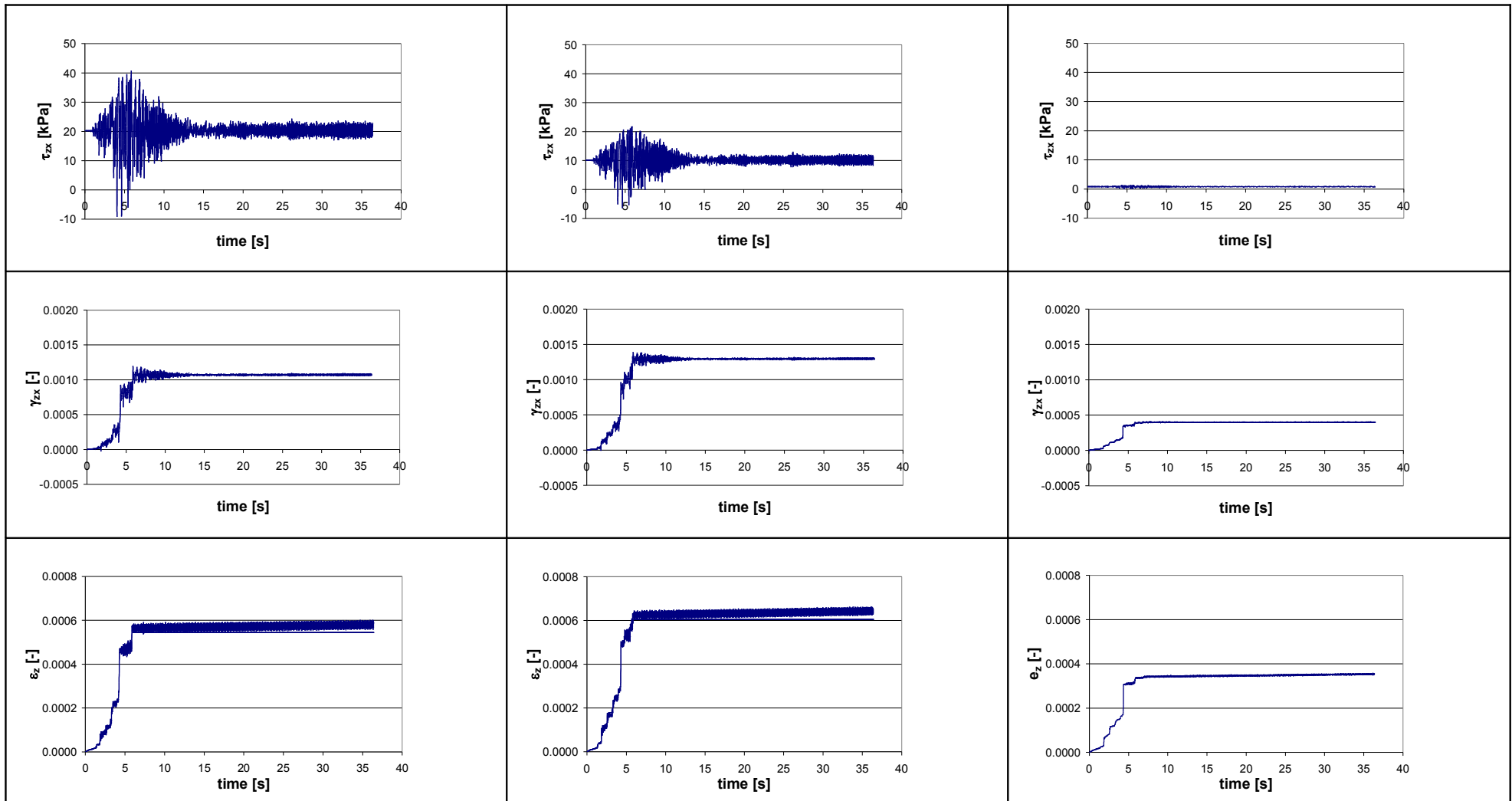
Figure 5.2 (a). Tangential stress and strain, vertical strain (base, middle and top of the layer), Toyoura sand.
