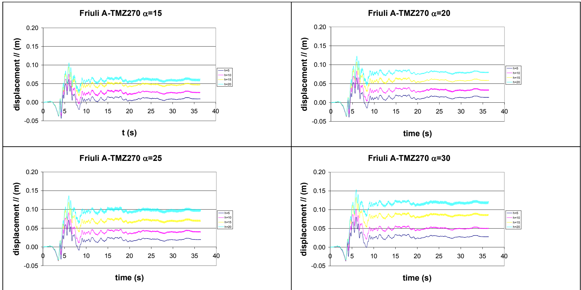
Figure 5.5. Permanent horizontal displacement, accelerometer A-TMZ270, soil type A, Toyoura sand.
