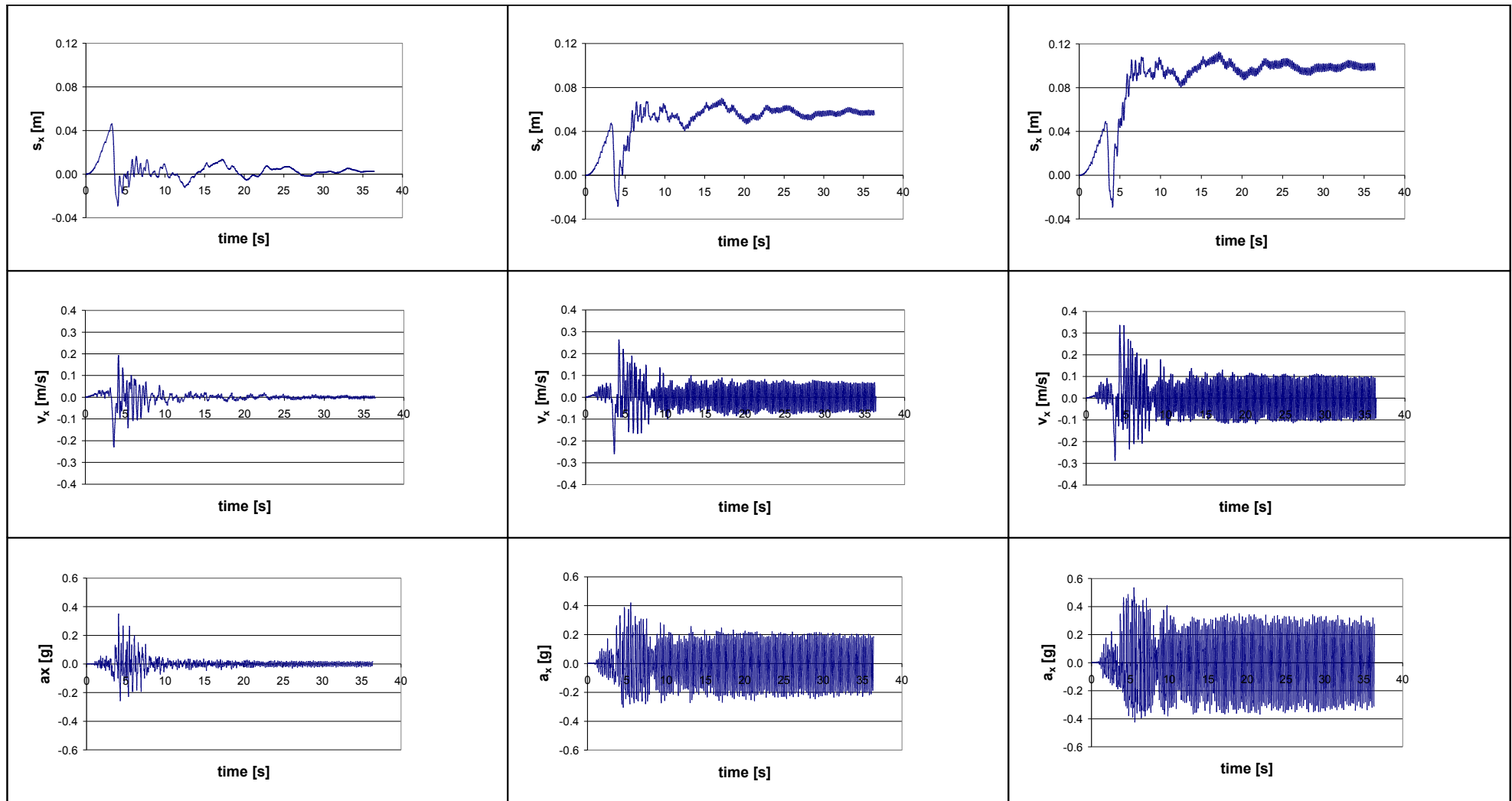
Figure 4.2 (c). Displacement, velocity and acceleration in x direction (base, middle and top of the layer), Hostun sand.
