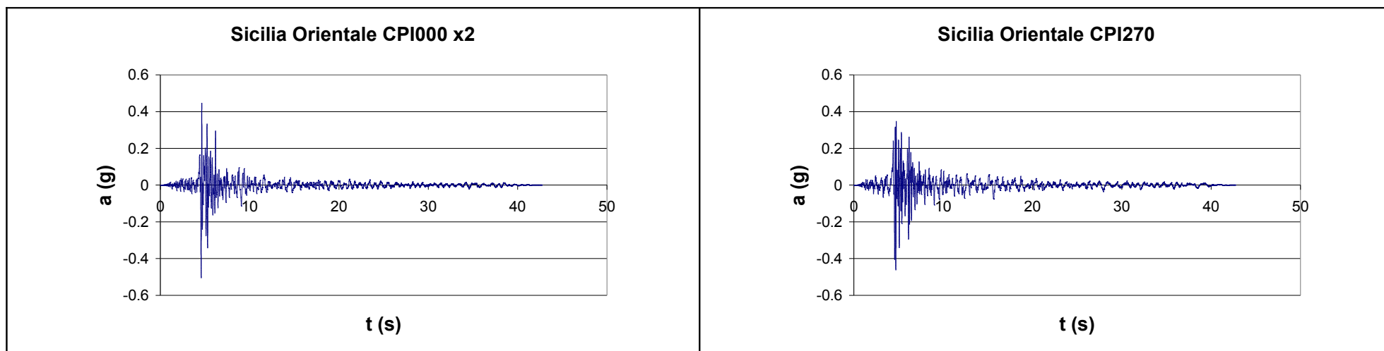
Figure 3.4 c. Strong motion accelerograms (amplified or not), site classification C: Sicilia Orientale earthquake, Catania - Piana station (NS-WE).
