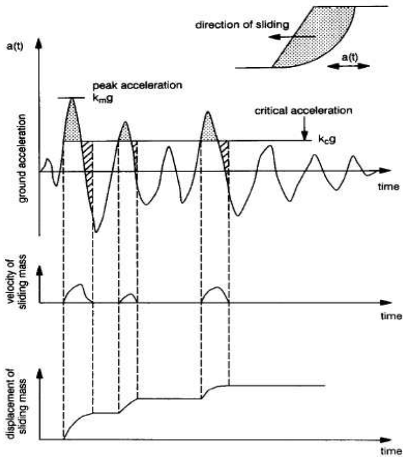
Fig. 1. Illustration of Newmark's sliding block method to calculate permanent displacement of earth structures (unsymmetrical displacement).
