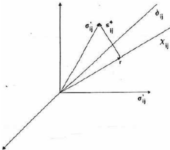
Figure 2.5 Stress space – definition of stress variables (di Prisco, 1993).
