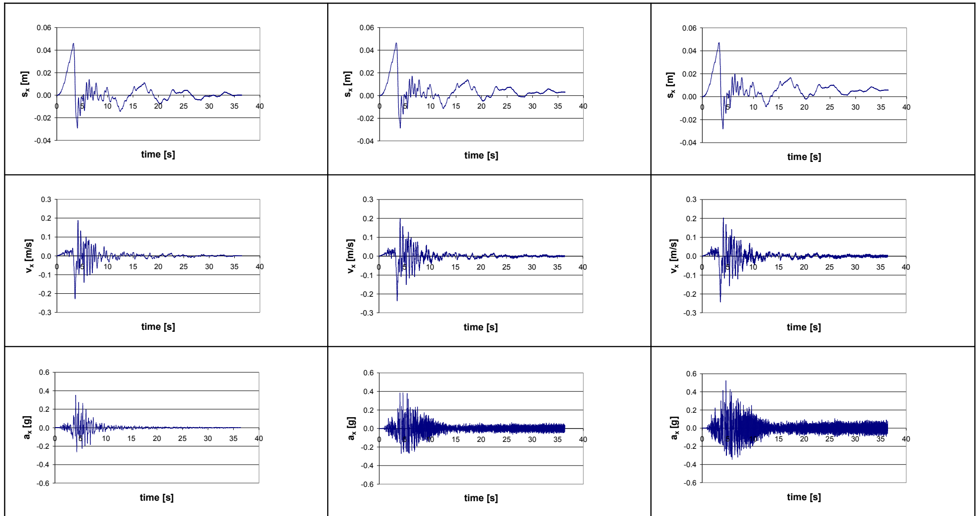
Figure 5.2 (c). Displacement, velocity and acceleration in x direction (base, middle and top of the layer), Toyoura sand.
