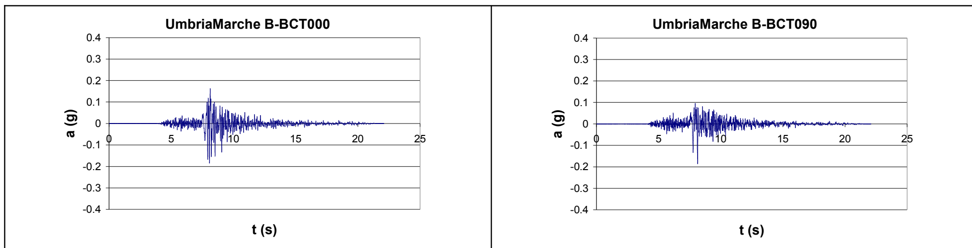
Figure 3.1 c. Strong motion accelerograms, site classification A: Umbria Marche 1 st earthquake, Borgo-Cerreto Torre station (NS-WE).
