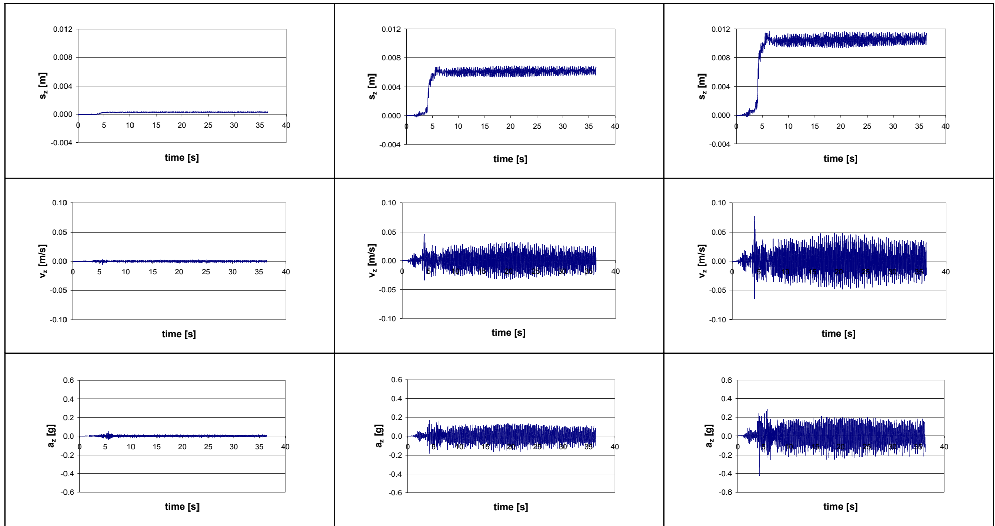
Figure 4.2 (d). Displacement, velocity and acceleration in z direction (base, middle and top of the layer), Hostun sand.
