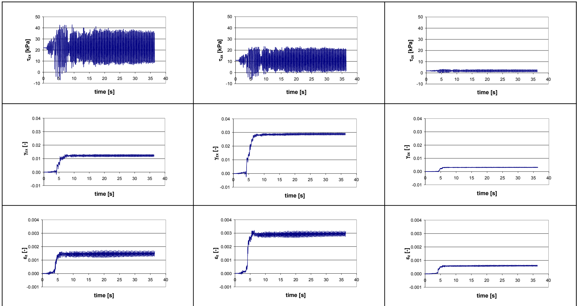
Figure 4.2 (a). Tangential stress and strain, vertical strain (base, middle and top of the layer), Hostun sand.
