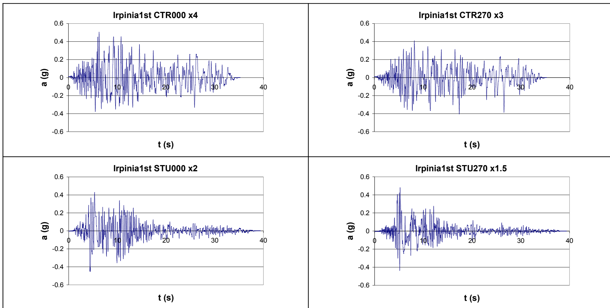
Figure 3.2 a. Strong motion amplified accelerograms, site classification A: Irpinia 1 st earthquake, Calitri and Sturno station (NS-WE).
