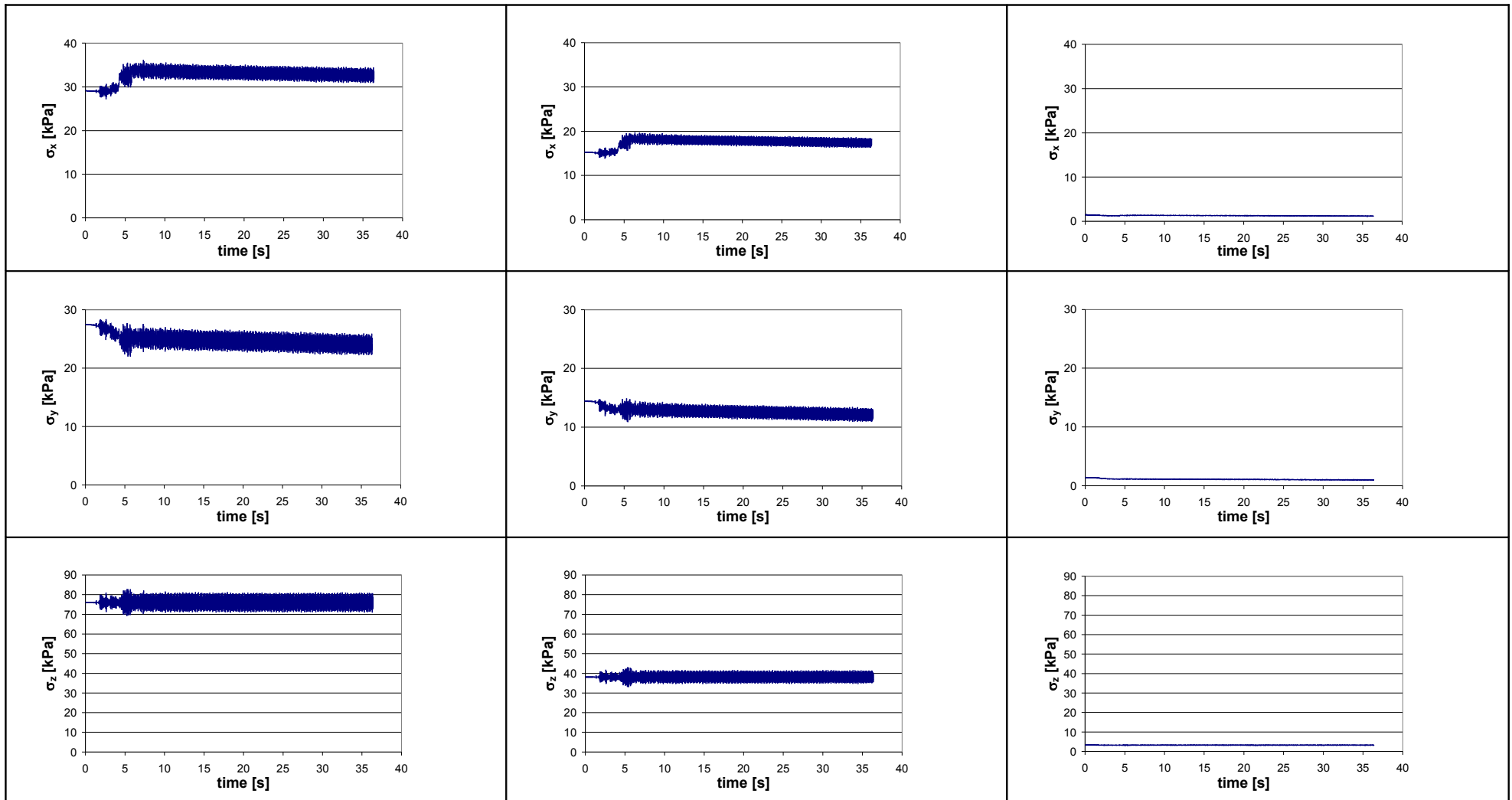
Figure 5.2 (b). Stress in x, y and z direction (base, middle and top of the layer), Toyoura sand.
