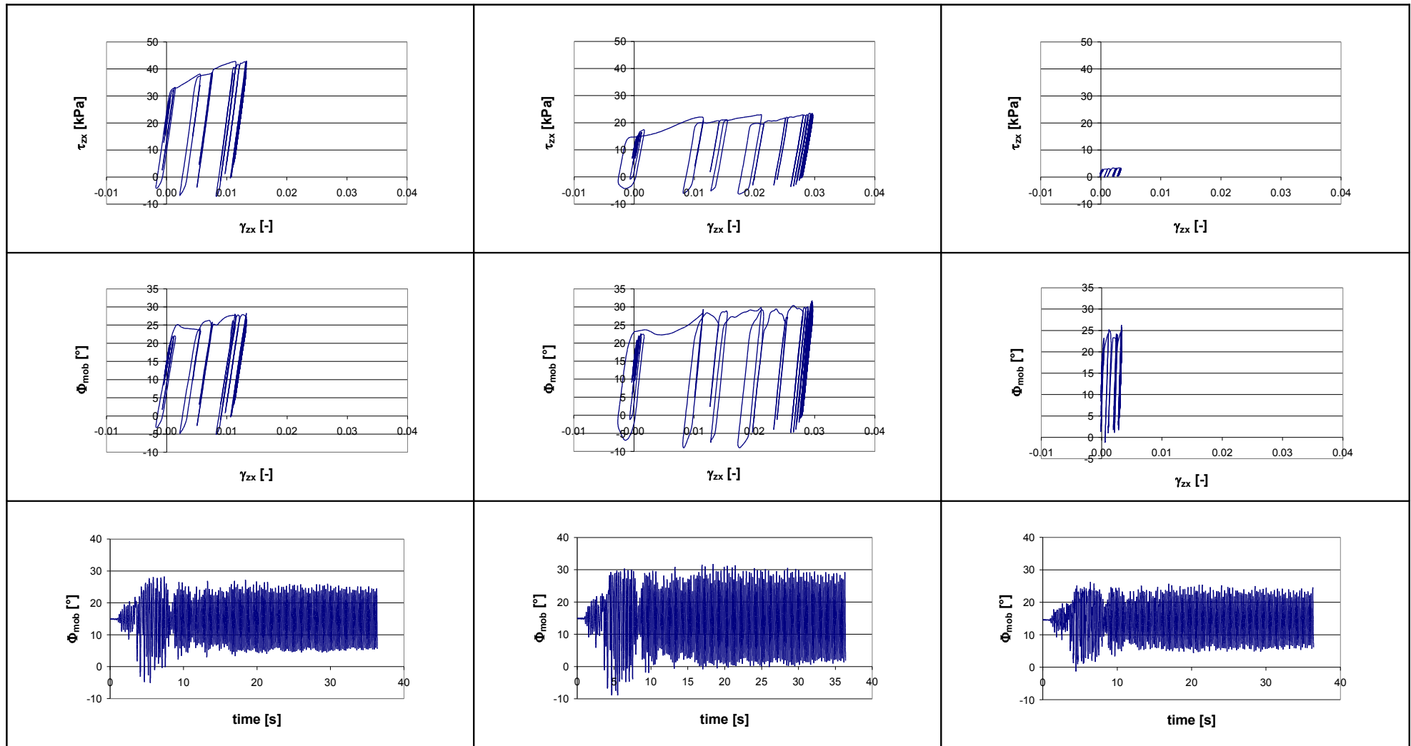
Figure 4.2 (e). Loading cycles and friction angle (base, middle and top of the layer), Hostun sand.
