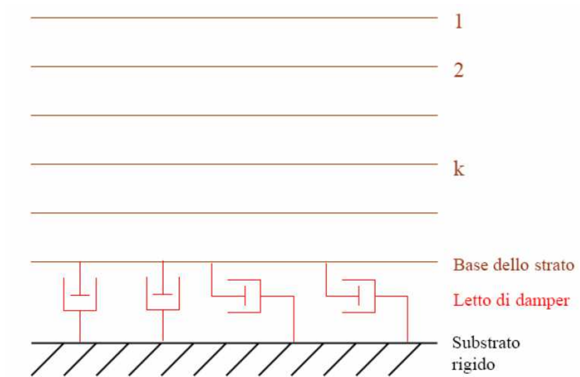
Figure 2.12. Scheme of the placement of the dampers at the interface between layer and bedrock.
