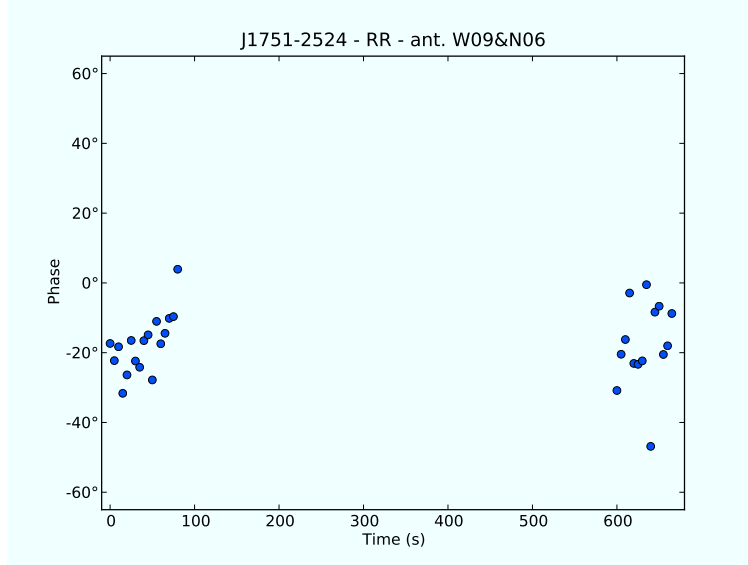
Figure 2.4: phase variations for two adjacent scans of the gain calibrator (the target source was acquired between this two scans). It is possible to notice that the phase fluctuations within one single scan are not completely negligible.
