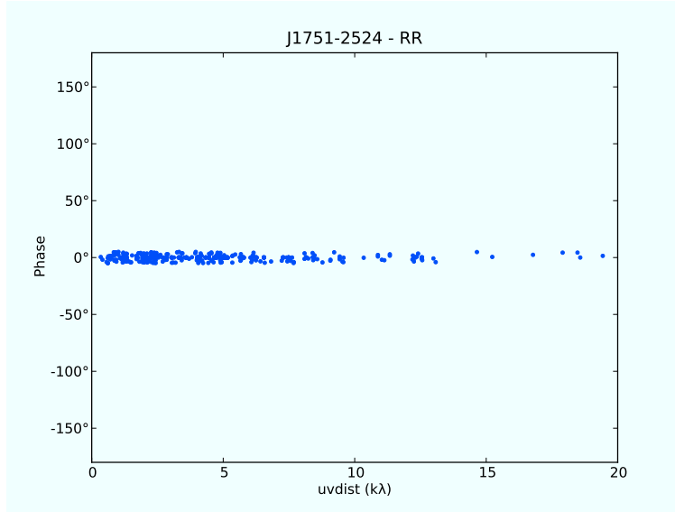
Figure 2.5: calibrated phase values for the gain calibrator J1751–2524 (only one spectral window and polarization are shown).
