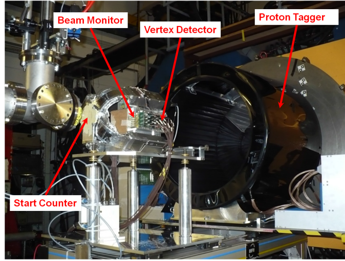
Figure 2.3.2: Picture of the Interaction Region, embedding the Start Counter, the Beam Monitor, the Vertex Detector and the Proton Tagger. The Interaction Region is located at the entrance of the ALADiN magnet.
