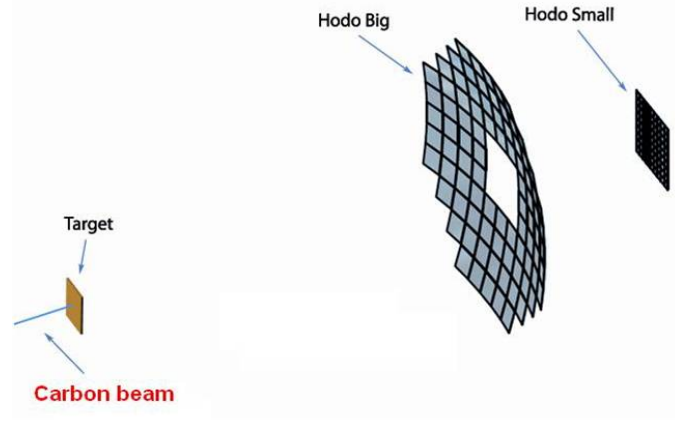
Figure 2.1.1: A schematic view of the FRAG experimental set-up at LNS.
