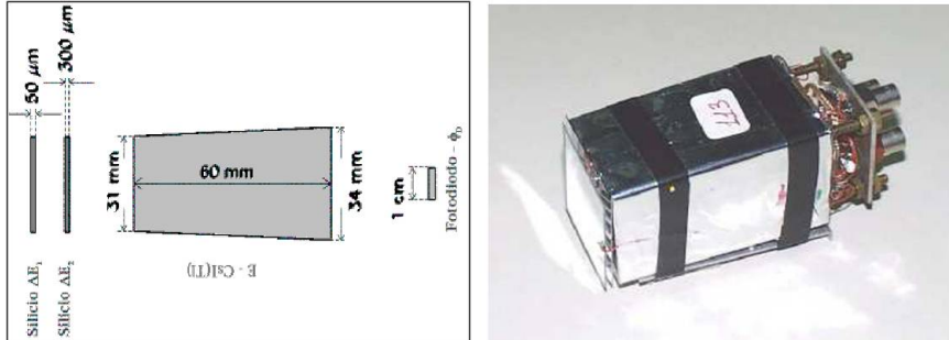
Figure 2.1.3: Schematic representation (left) and image (right) of a telescope of the Hodo-Big.
