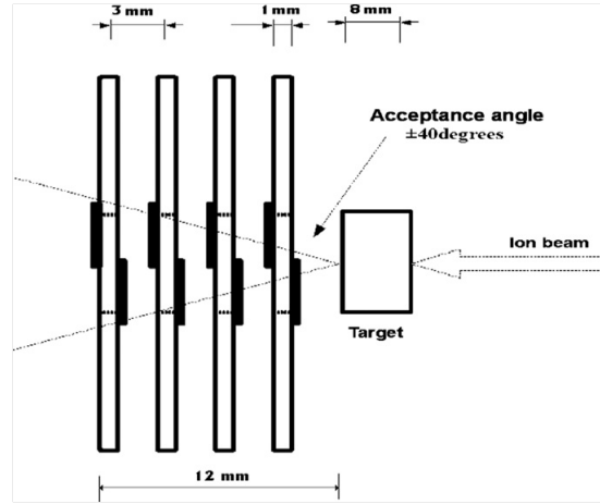
Figure 2.3.5: Relative positions of beam, target, four vertex stations and sensor housing board dimensions.
