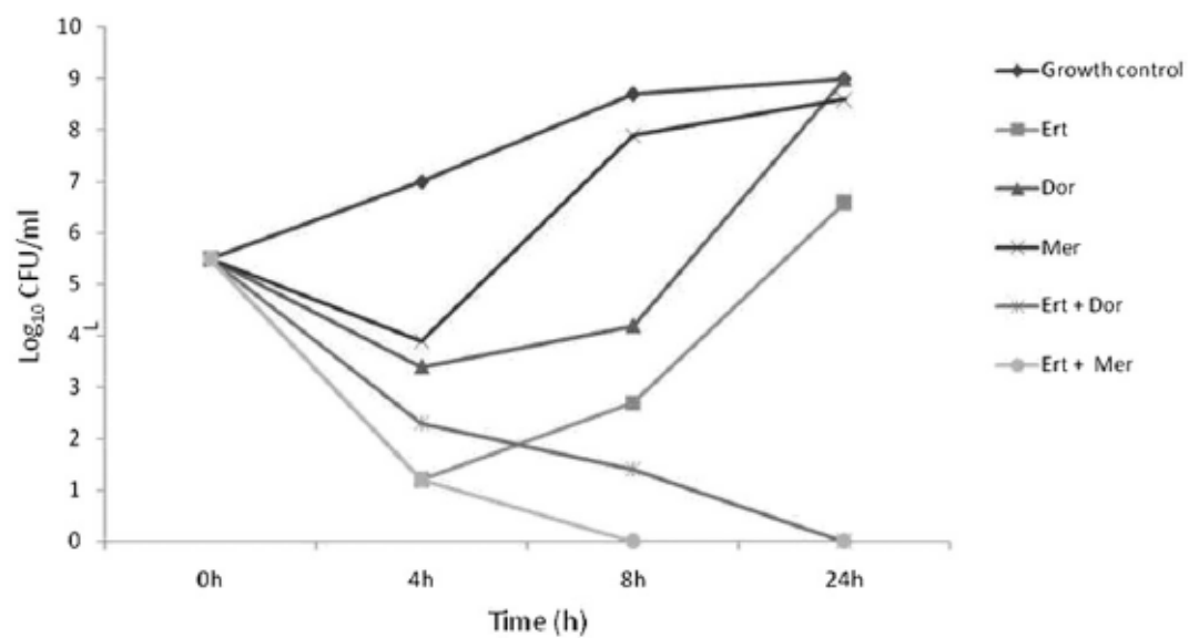
FIG4 Time-kill curves for K. pneumoniae with ertapenem (Ert) at 1 X MIC (512 mg/liter), doripenem (Dor) at 1 X MIC (64 mg/liter), meropenem (Mer) at 1 X MIC (64 mg/liter), and the combinations of ertapenem plus doripenem at 1 X MIC and ertapenem plus meropenem at 1 X MIC.
