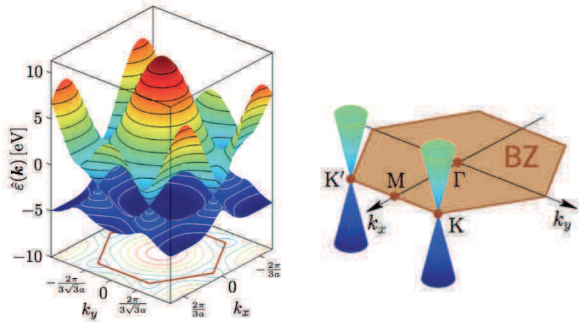
Fig. 1.4 Energy bands in graphene
