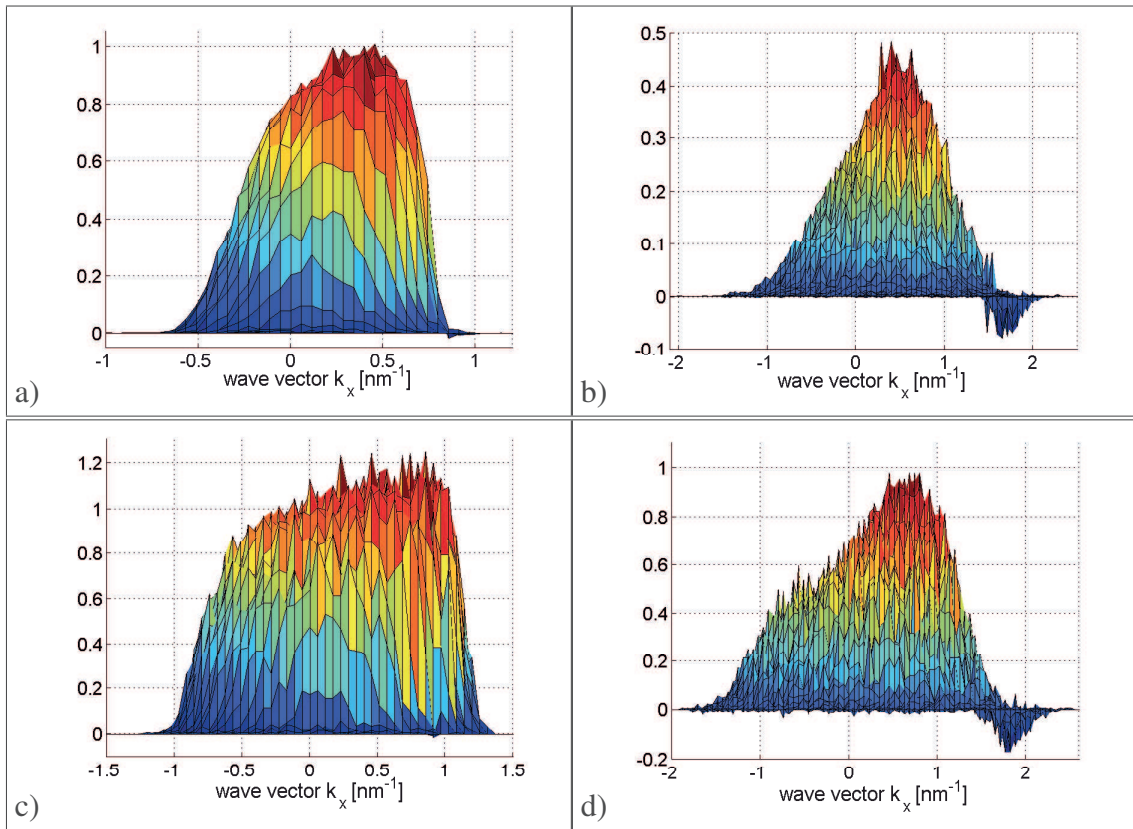
Fig. 2.20 Distribution function section along the field direction with variant 1. \epsilon_F = 0.3 eV and E = 2 kV/cm a), \epsilon_F = 0.3 eV and E = 20 kV/cm b), \epsilon_F = 0.6 eV and E = 2 kV/cm c), \epsilon_F = 0.6 eV and E = 20 kV/cm d).
