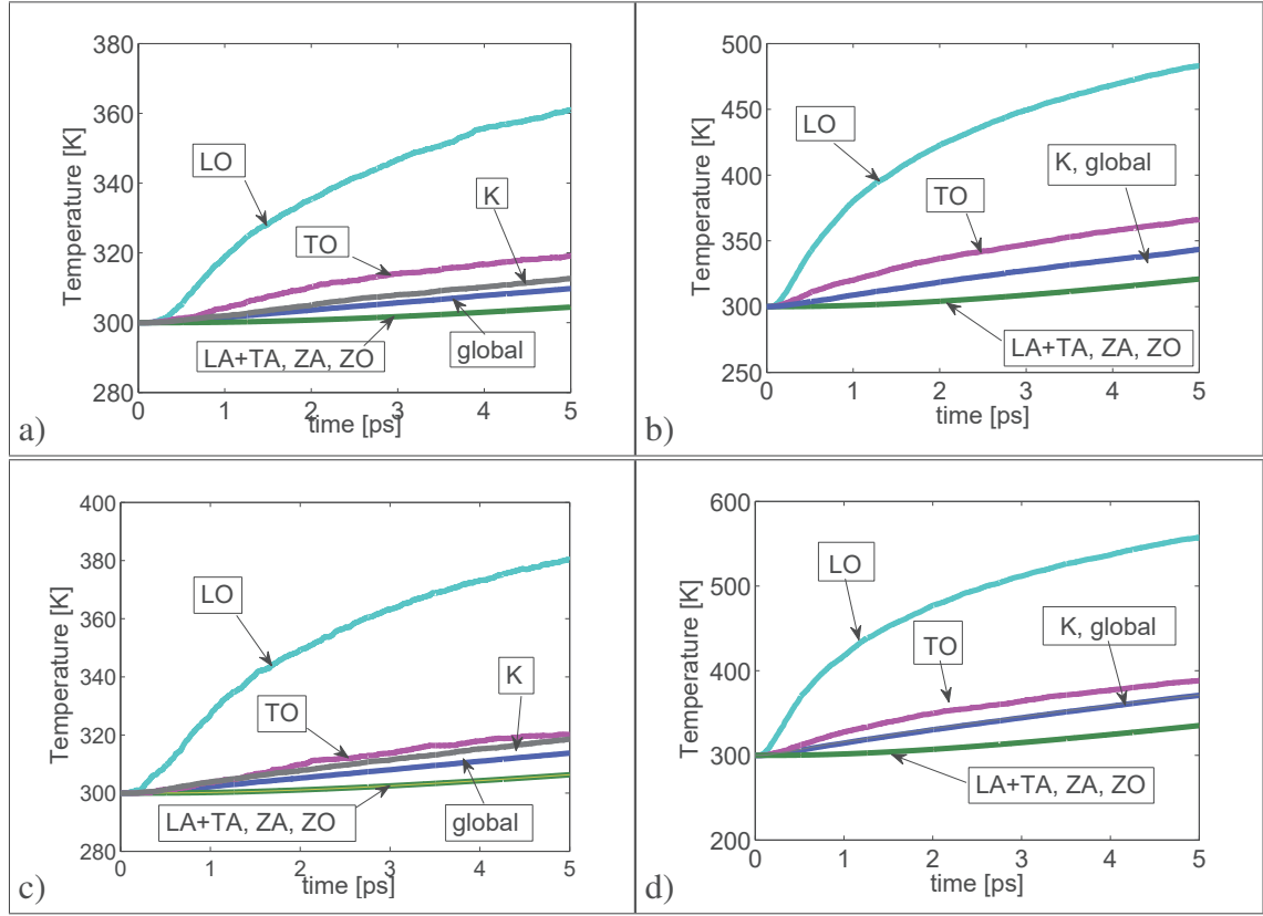
Fig. 5.2 Phonon temperatures and local equilibrium temperature T_{LE} versus time in the case \epsilon_F = 0.4 eV when E = 5 kV/cm (a), E = 20 kV/cm (b), and in the case \epsilon_F = 0.6 eV when E = 5 kV/cm (c) and E = 20 kV/cm (d).
