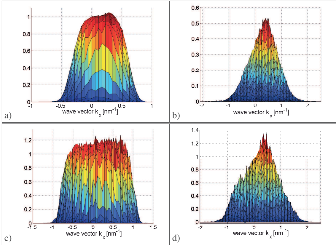
Fig. 2.25 Distribution function section along the field direction with variant 3. \epsilon_F = 0.3 eV and E = 2 kV/cm a), \epsilon_F = 0.3 eV and E = 20 kV/cm b), \epsilon_F = 0.6 eV and E = 2 kV/cm c), \epsilon_F = 0.6 eV and E = 20 kV/cm d).
