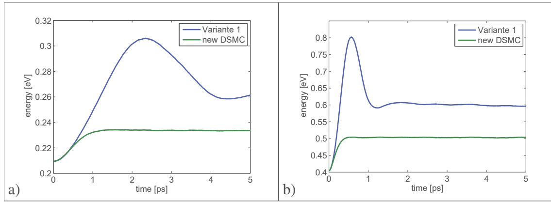
Fig. 2.18 Comparison of the average energy versus time obtained with the variante 1 and the new DSMC when E = 2 kV/cm and \epsilon_F = 0.3 eV a), and when E = 20 kV/cm and \epsilon_F = 0.6 eV b).
