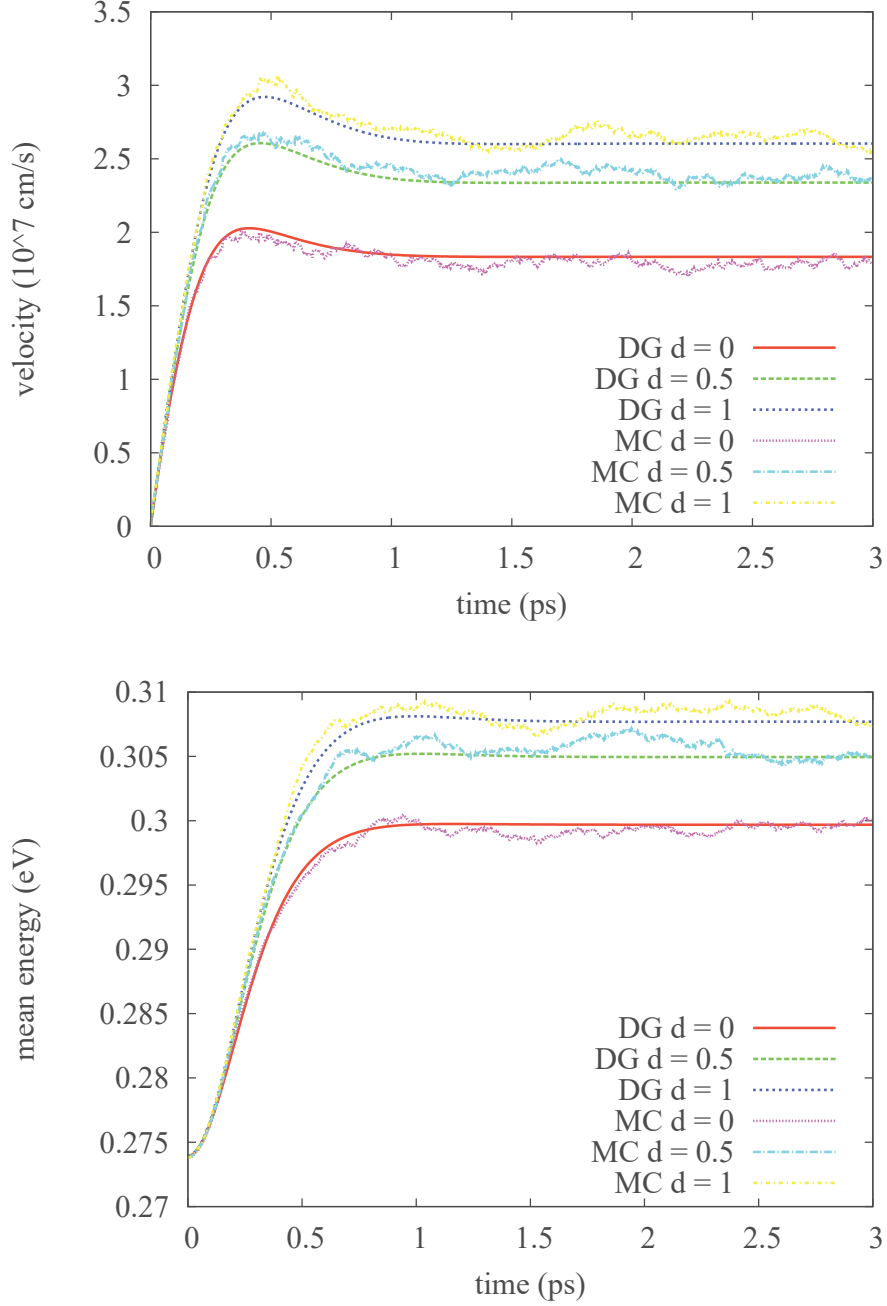
Fig. 4.3 Comparison of the average velocity (top) and average energy (bottom) versus time for d = 0, 0.5, 1 nm in the case of an applied electric field of 5 kV/cm and Fermi energy \epsilon_F = 0.4 eV.
