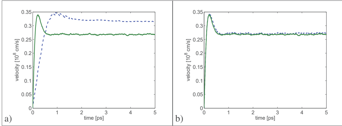
Fig. 2.24 Comparison of the average velocity versus time obtained with the variant 3 (dashed line) and the new DSMC (continuous line) when E = 2 kV/cm and \epsilon_F = 0.3 eV a), and when E = 20 kV/cm and \epsilon_F = 0.6 eV b).
