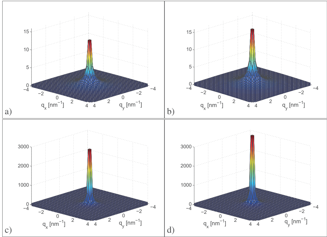
Fig. 5.6 initial (LA + TA) distribution (a), final (LA + TA) distribution after 10 ps (b), initial ZA distribution (c), final ZA distribution after 10 ps (d), in the case \epsilon_F = 0.6 eV and E = 20 kV/cm.
