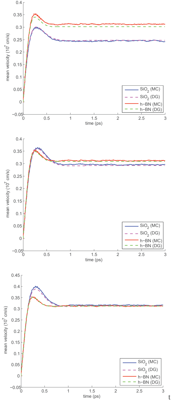
Fig. 4.7 Comparison of the average velocity versus time for d = 0 (top) , 0.5, 1 (bottom) nm in the case of an applied electric field of 10 kV/cm and Fermi energy \varepsilon_F = 0.4 eV.
