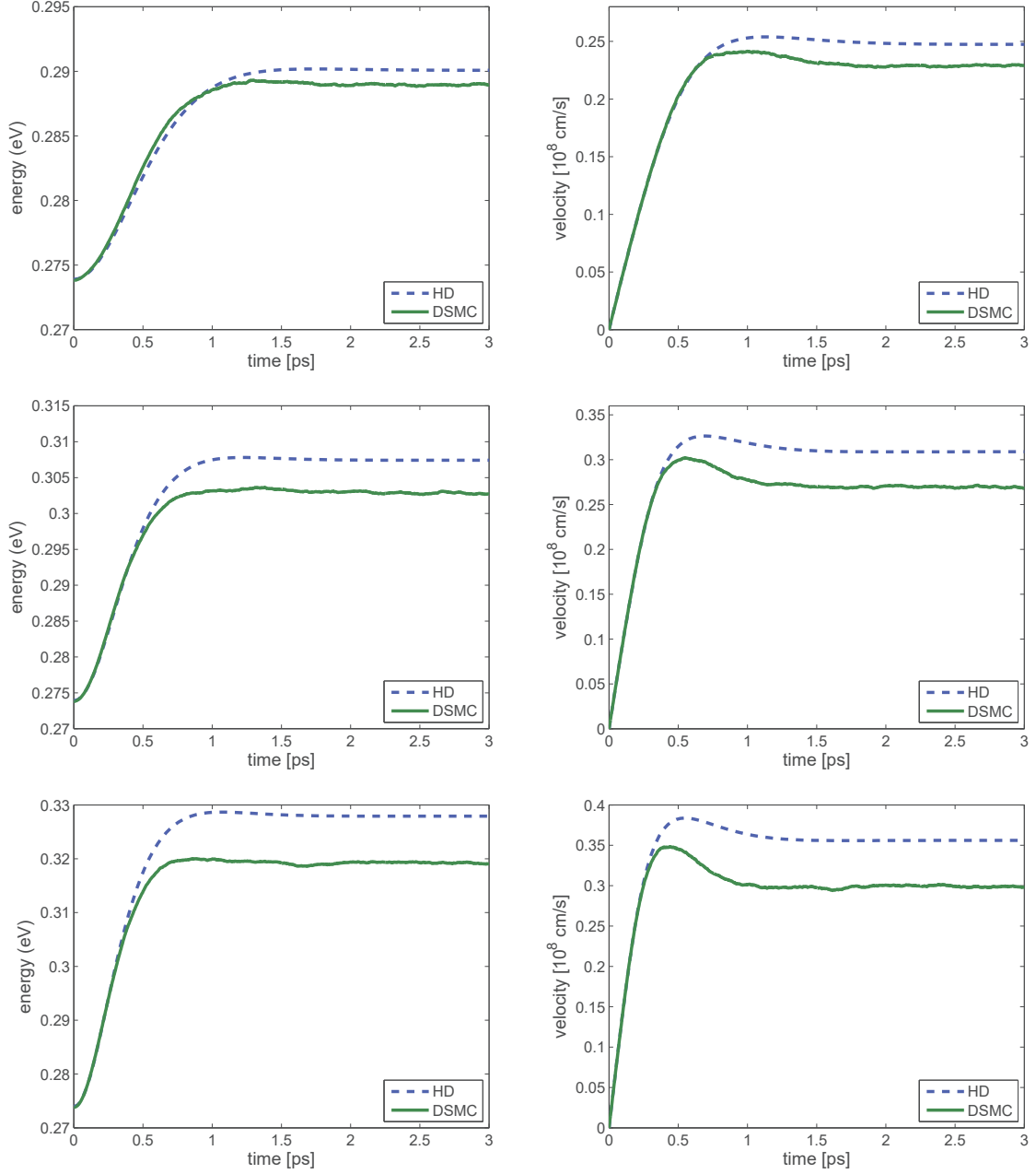
Fig. 6.1 Comparison of the energy and the velocity versus time obtained with DSMC and the MEP hydrodynamical model (HD) for the electric fields E = 2 kV/cm (top), E = 4 kV/cm, E = 6 kV/cm (bottom) and a Fermi energy equal to 0.4 eV.
