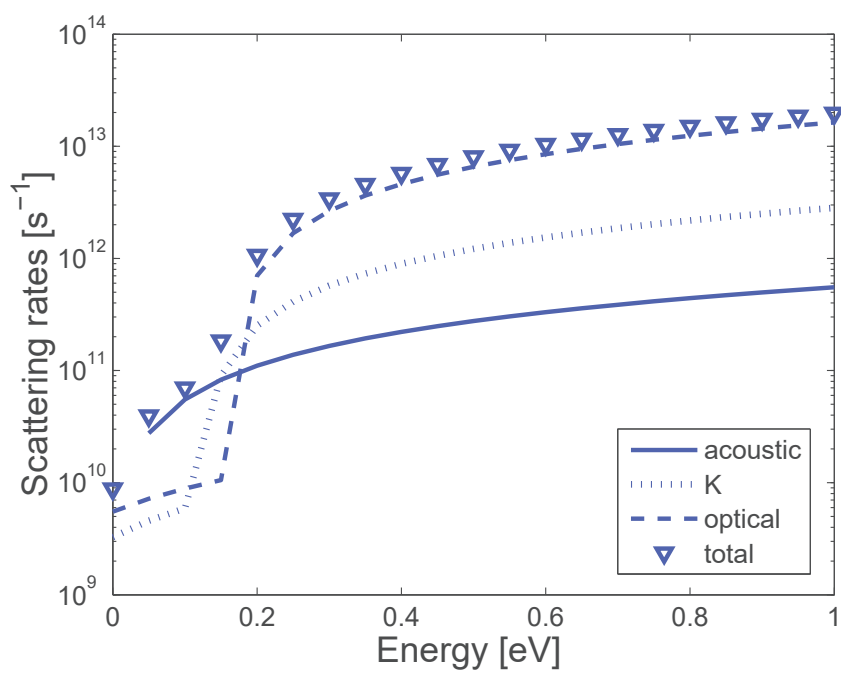
Fig. 1.5 Scattering rates.
