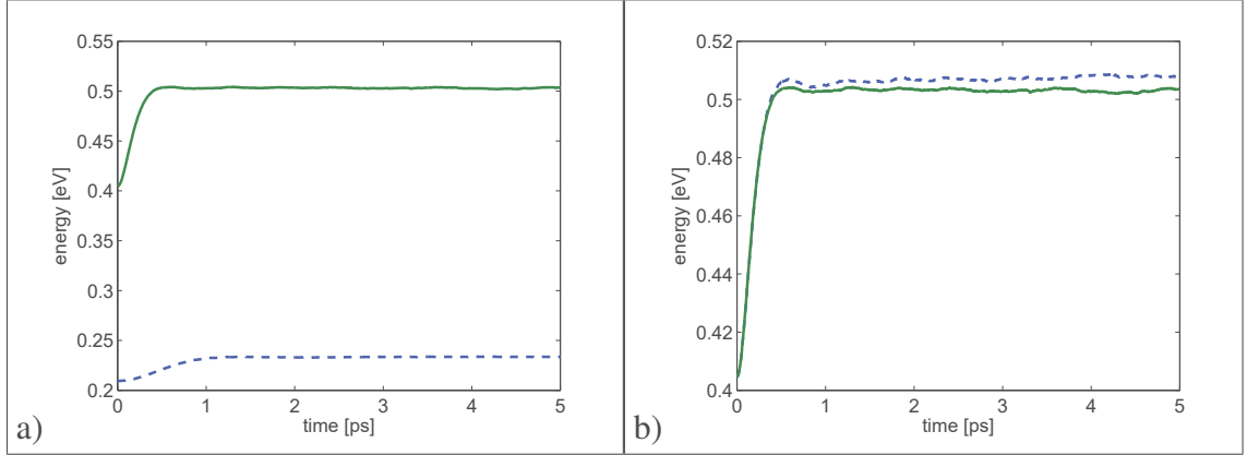
Fig. 2.23 Comparison of the average energy versus time obtained with the variant 3 (dashed line) and the new DSMC (continuous line) when E = 2 kV/cm and \epsilon_F = 0.3 eV a), and when E = 20 kV/cm and \epsilon_F = 0.6 eV.
