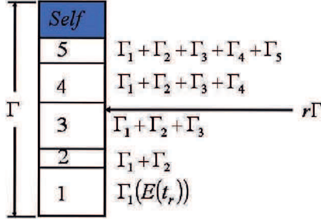
Fig. 2.3 Selection of the scattering mechanism terminating the free flight.
