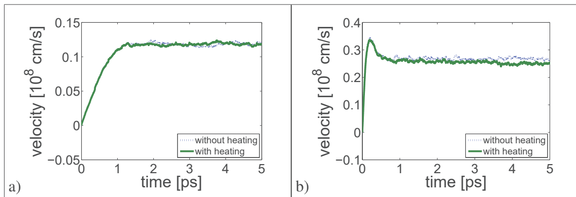
Fig. 5.23 Average electron velocity versus time in the case \varepsilon_F = 0.6 eV, when E = 1 kV/cm (a) and E = 20 kV/cm (b).
