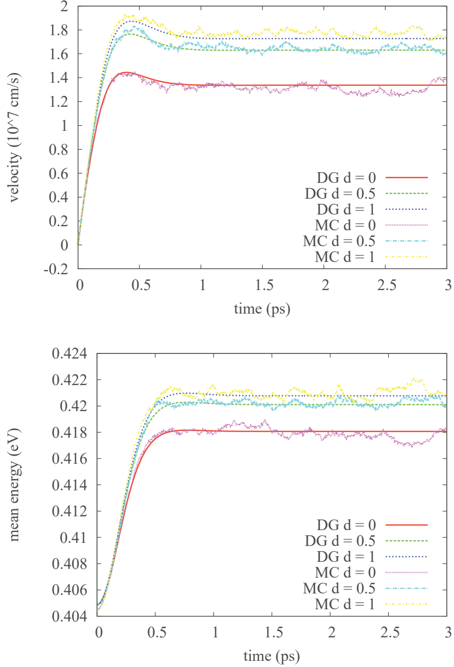
Fig. 4.5 Comparison of the average velocity (top) and average energy (bottom) versus time for d = 0, 0.5, 1 nm in the case of an applied electric field of 5 kV/cm and Fermi energy \epsilon_F = 0.6 eV.
