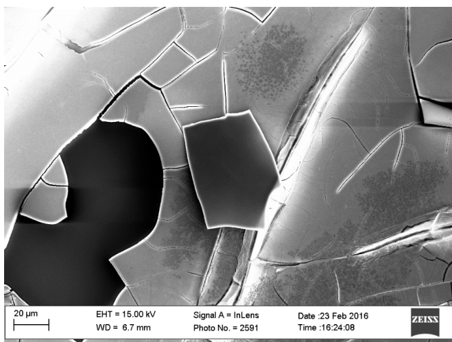
Fig. 28: TiLi(5)Ce(3)-NS nanosheets.
