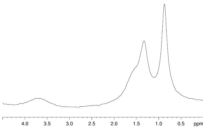
Fig. C: ^1\text{H} MAS NMR of the sample \text{TiLi}(5)\text{Co}(5) , peaks: 0.88, 1.36, 1.61, 3.70 ppm.
