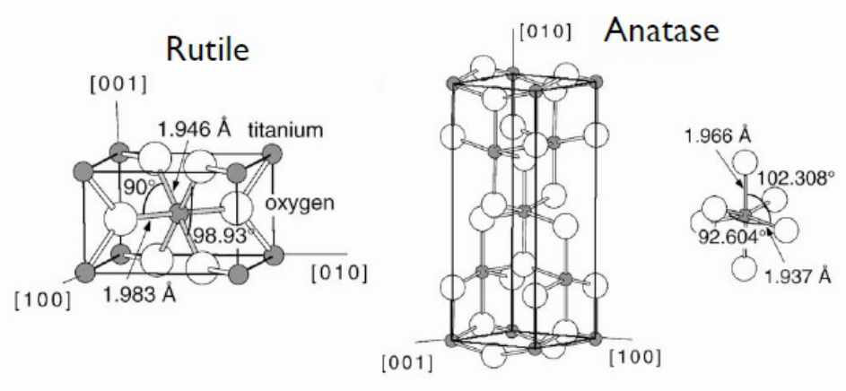
Fig. 5: Bulk structure of rutile and anatase. The tetragonal bulk unit cell of rutile has the dimensions a = b = 4.857 \text{ \AA} , c = 2.953 \text{ \AA} and the one of anatase a = b = 3.782 \text{ \AA} , c = 9.502 \text{ \AA} . In both structures, slightly distorted octahedra constitute the basic building units [36].
