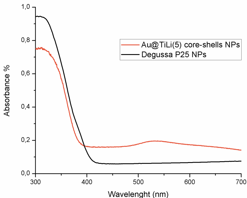
Fig. 58: Comparison of the absorption spectra of Degussa P25 NPs (black) and the Au@TiLi(5) core-shells NPs (orange).
