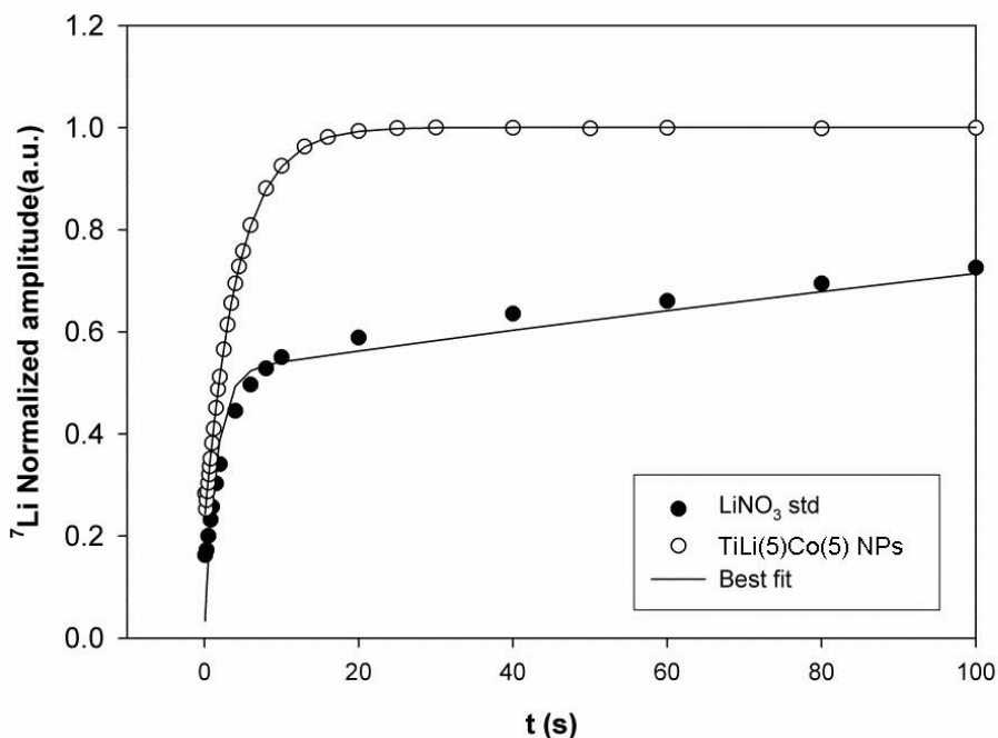
Fig. 53: Longitudinal relaxation decay measured in \text{LiNO}_3 (black circles) and Li-doped \text{TiO}_2 nanoparticles with \text{CoCl}_2 and \text{LiNO}_3 (white circles).
