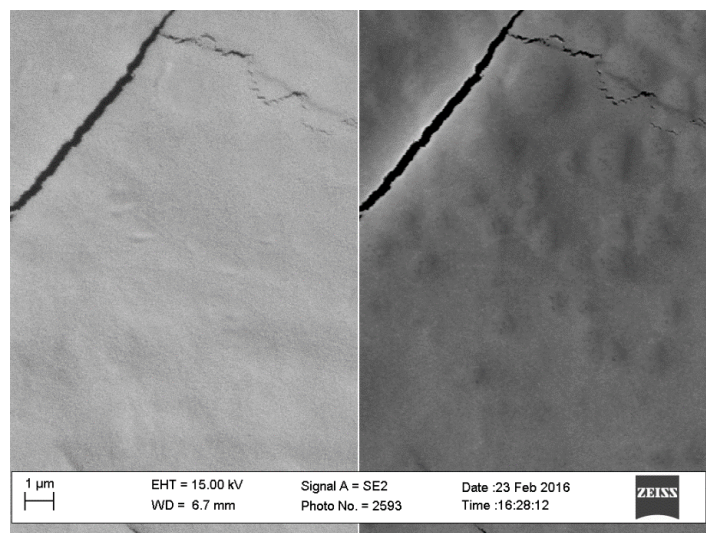
Fig. 29: TiLi(5)Ce(3)-NS nanosheets.
