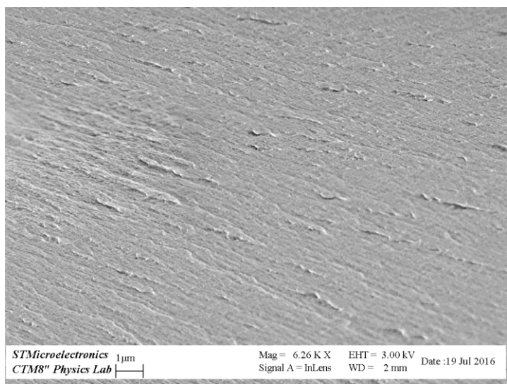
Fig. 30: TiLi(5)Co(5)-NS nanosheets.
