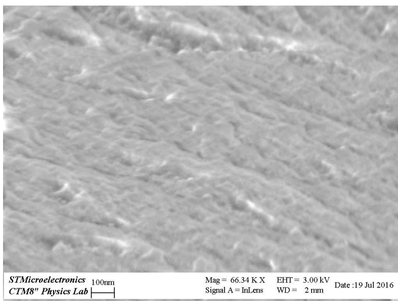
Fig. 32: TiLi(5)Co(5)-NS nanosheets.
