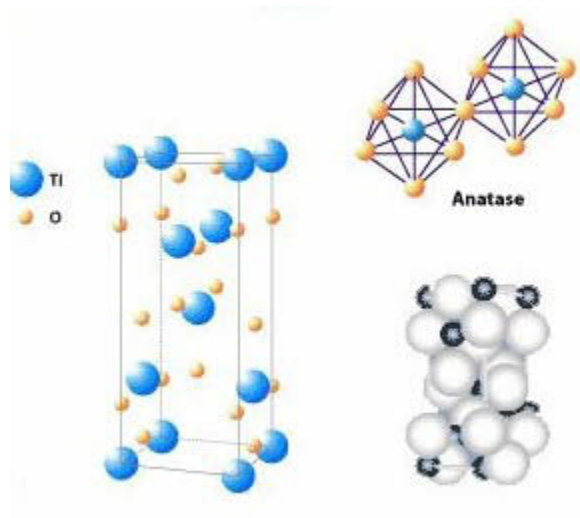
Fig. 4: Anatase structure.
