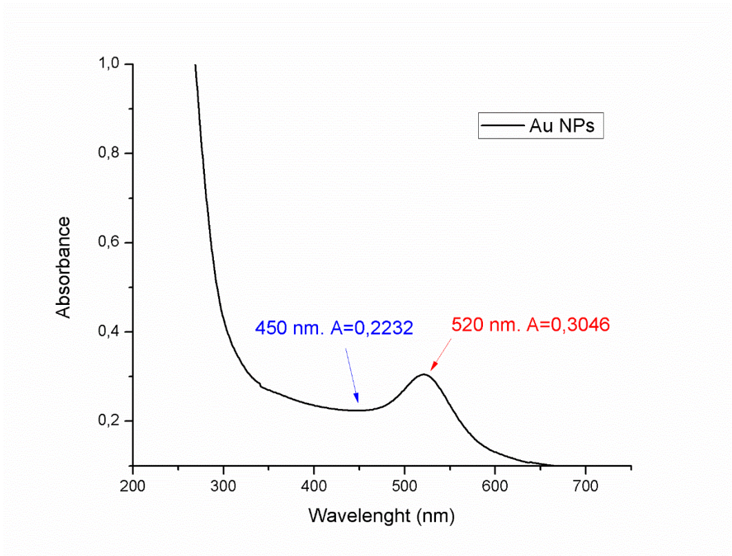
Fig. 22: Plasmon resonance of the Au NPs, solution diluted 10 times.
