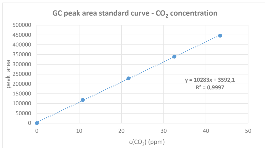
Fig. 86: Gas chromatography standard curve for CO 2 .
