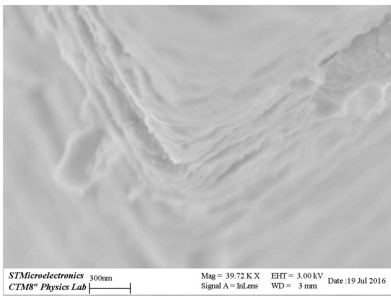
Fig. 31: TiLi(5)Co(5)-NS nanosheets.
