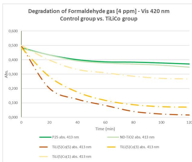
Fig. 83: Degradation of HCHO under visible light and comparison between the control group and the TiLiCo group.
