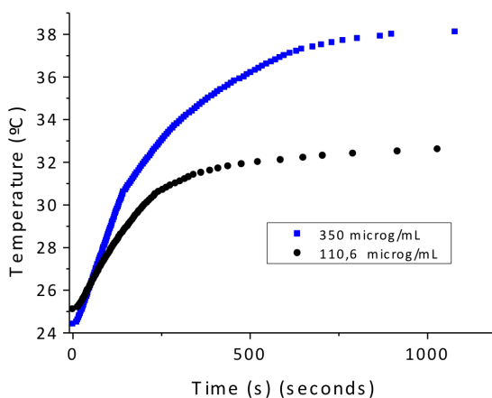
FIGURE 3.10: Increase of temperature depending on irradiation time with 532 nm laser (200 mW) of GO 1.5 mL in a Eppendorf.
