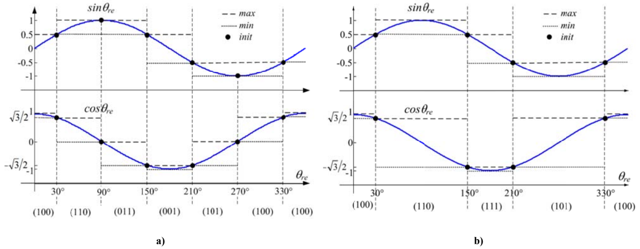
Figure 5.20 HOS for: a) normal operation, b) H_I=1 fault.
