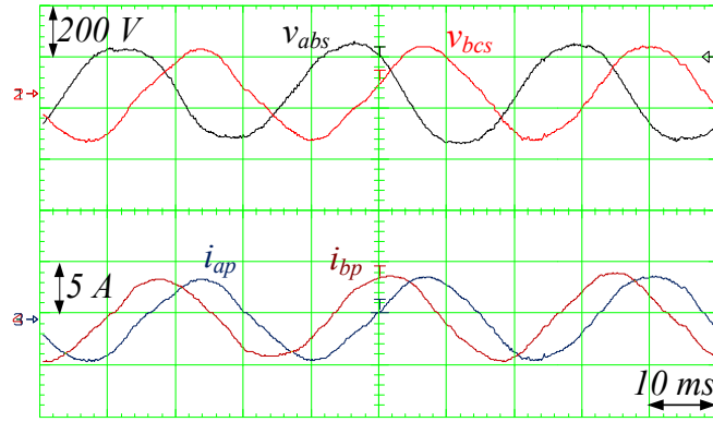
Figure 3.33 Steady state test with transformer operating in faulty conditions, at 50% of the rated load: Line to line voltages v_{abstr} , v_{bcstr} at the secondary windings and phase currents i_{aptr} , i_{bptr} at the primary windings.
