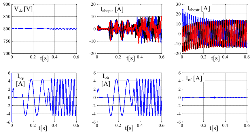
Figure 3.26 Performance evaluation of the Grid side system under phase c fault on the PMSG.
