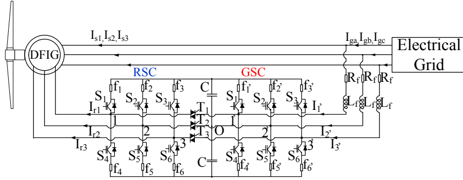
Figure 3.11 Fault tolerant topology without redundancy.
