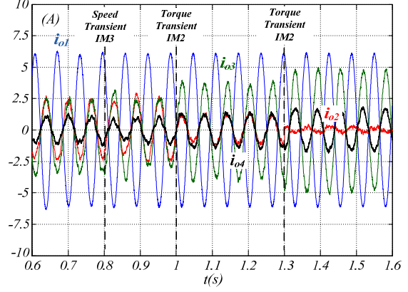
Figure 4.15 Zero-sequence currents flowing in each motor when applying the third method \hat{i}_{s3} = 1.5i_{s3} .
