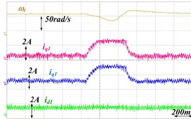
Figure 2.21 Load transient T_{\text{total\_load}} = 100\% T_{\text{en}} , \omega_r = 70 rad/s. The two motors are operating under single open phase fault in each motor and controlled by imposing \theta_{\lambda r1} = \theta_{\lambda r2} .
