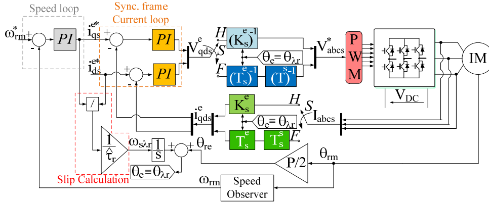
Figure 1.34 Fault tolerant control block diagram for Rotor Flux Indirect Field Orientation.
