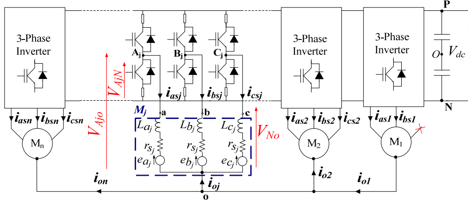
Figure 2.5 MDS with one drive working in fault conditions with all the neutral point connected together.
