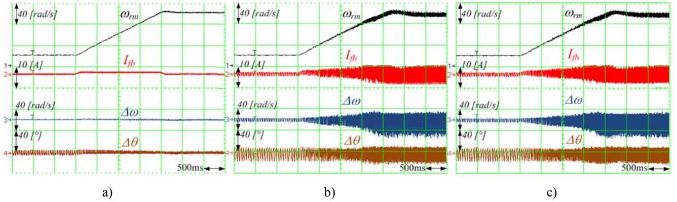
Figure 5.29 Position sensors misalignment 120^\circ+5^\circ H_2 and -5^\circ H_3 : a) VTO b) ZOA c) HO.
