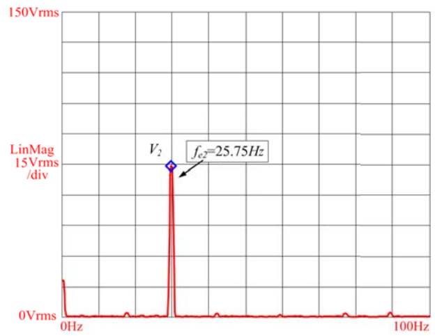
B) Phase voltage measured in IM_2 .
