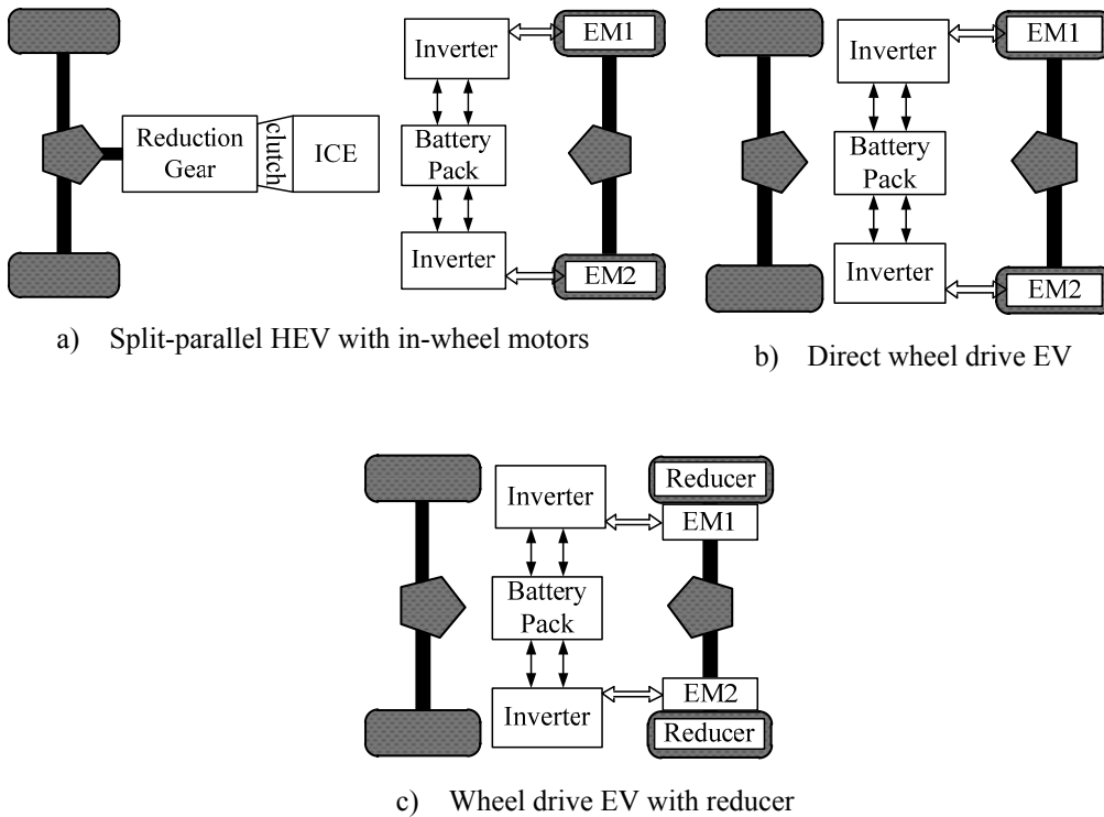
Figure 1.3 Wheel drive systems for HEV and EV.
