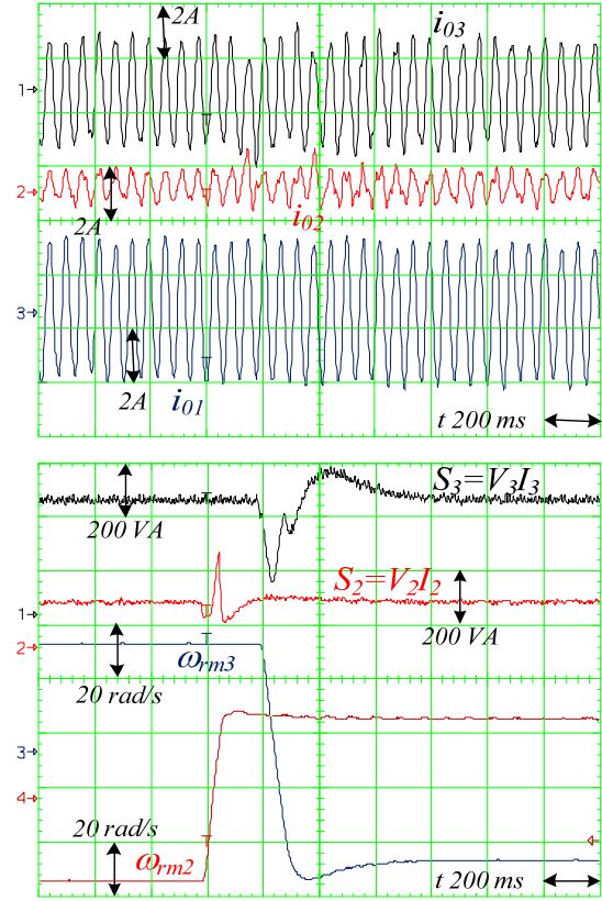
Figure 2.10 First method: Speed transients occurring at IM 2 : \omega_{rm\_IM2}=30/30 \text{ rad/s} and IM 3 : \omega_{rm\_IM3}=40/-40 \text{ rad/s} , while IM 1 operates at \omega_{rm\_IM1}=50 \text{ rad/s} .
