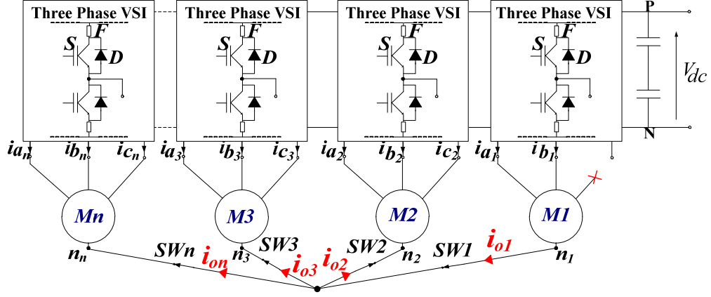
Figure 4.2 Post fault configuration of the MDS.
