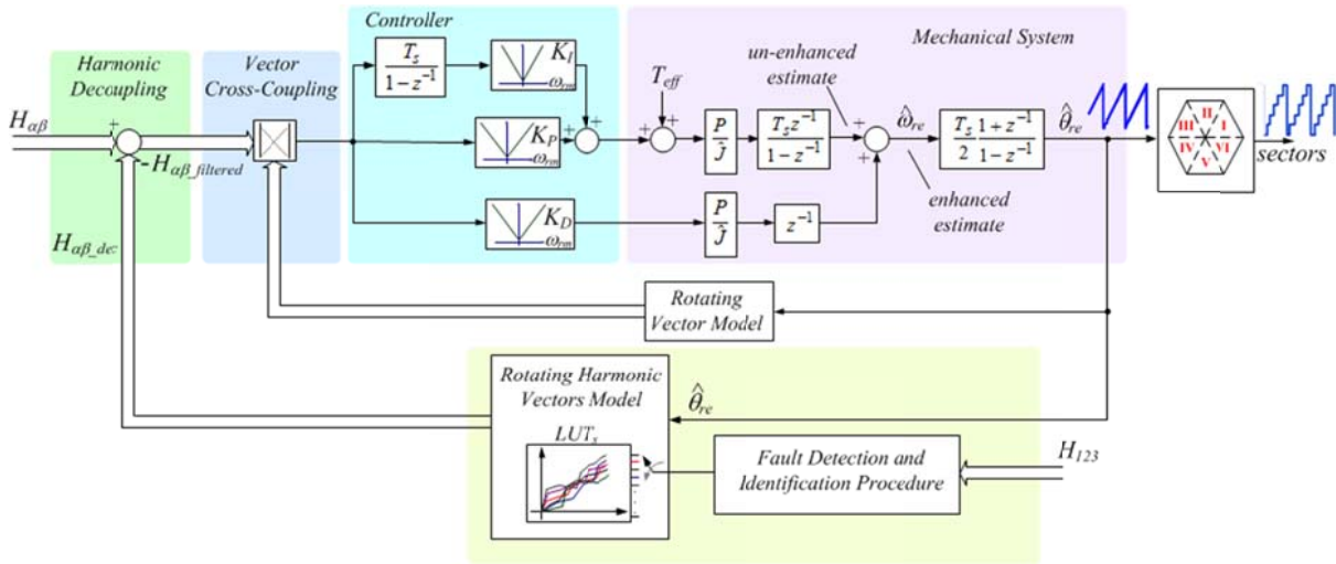
Figure 5.14 B block diagram of the fault tolerant vector tracking observer with harmonic decoupling.
