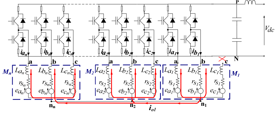
Figure 2.2 Sharing current strategy in case of a single faulted drive.
