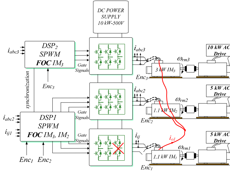
Figure 4.16 Experimental setup.
