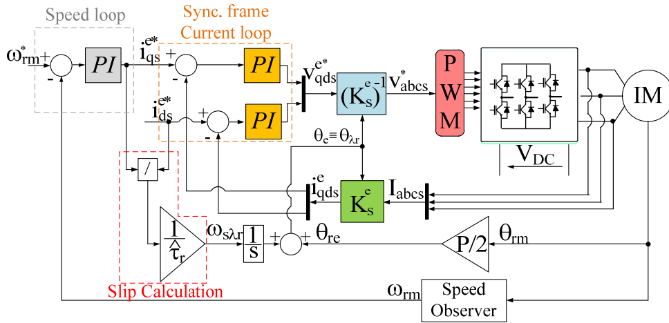
Figure 1.33 Block diagram of the Rotor Flux Field Oriented Control for IM.
