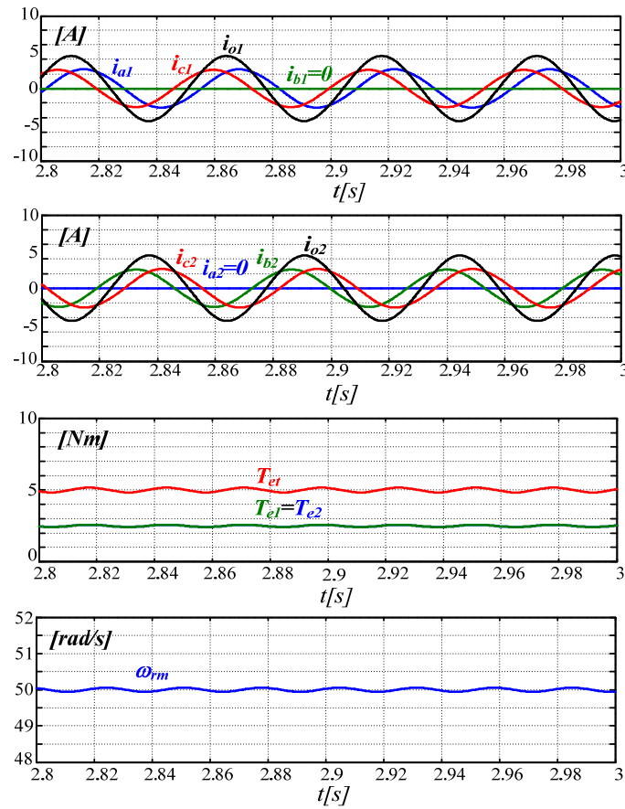
Figure 2.15 Two single open phase faults.
