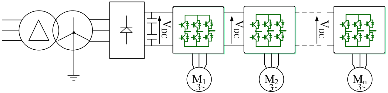
Figure 1.5 Standard three phase MDS topology.
