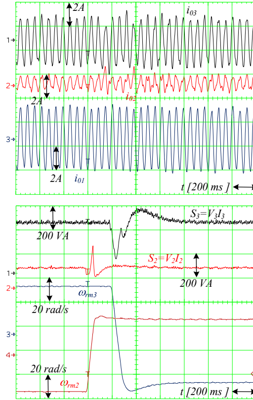
Figure 4.19 First method: speed transients occurring at: IM 2 : \omega_{rm\_IM2} = -30/30 \text{ rad/s} and IM 3 \omega_{rm\_IM3} = -40/40 \text{ rad/s} , whereas IM 1 operates at \omega_{rm\_IM1} = 50 \text{ rad/s} .
