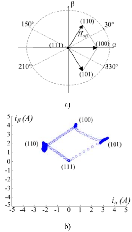
Figure 5.35 Quantized loci in the stationary reference frame for a H_l = 1 single fault: a) position vector H_{\alpha\beta} b) current vector i_{\alpha\beta} .
