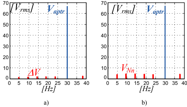
Figure 3.36 Harmonic spectrum of the phase voltage in the transformer and harmonic spectrum of V_{nN} : PMSG is controlled at different rotational speeds \omega_{rm} = 20 \div 80 rad/s, while the transformer is operating at f_e = 30 Hz and V_{ab\_rms} = 135 V.
