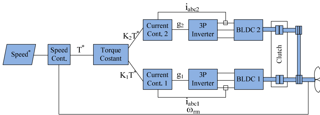
Figure 1.16 Coupled motors configuration for submarine application.
