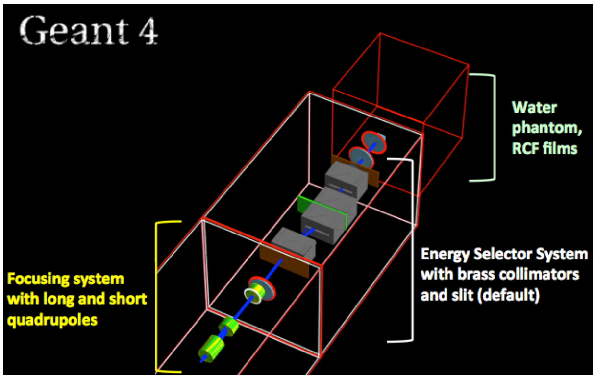
FIGURE 2.2: The transport beamline dedicated to laser-driven beams simulated with the Geant4 toolkit as an optional line of the hadrontherapy advanced example.
