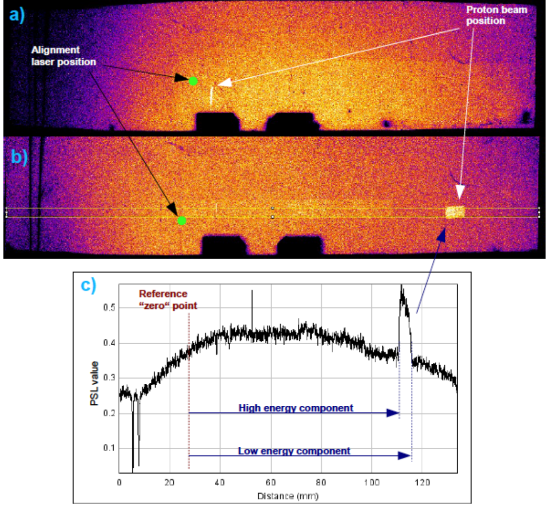
FIGURE 5.12: Measurement of: a) the zero point of the output beam respect to a fixed reference position (the laser alignment is the green point); b) the energy spread through the proton deflection due to the additional magnet. c) The IP signal analysis performed with the ImageJ tool. These data are obtained when 4.5 MeV was the selected energy.
