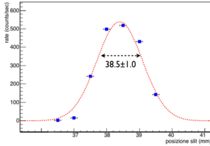
FIGURE 4.19: Detector counts versus slit position, with 0 as the input beam axis. The data set is referred to a 4.5 MeV proton beam delivered by the TANDEM with a fixed beam rate.
