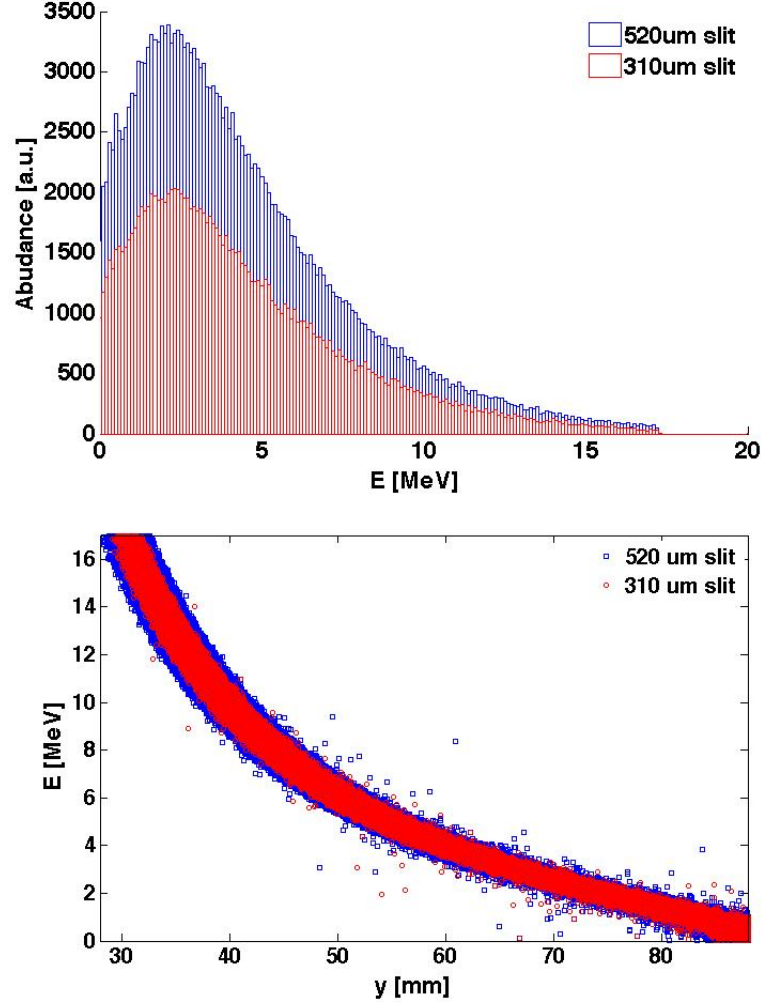
FIGURE 3.11: Energy spectra (top) and E vs y curves (bottom) obtained using 310 and 520 \mu\text{m} entrance slit apertures. The '1°' input exponential trend and a fixed number of simulated particles were used.
