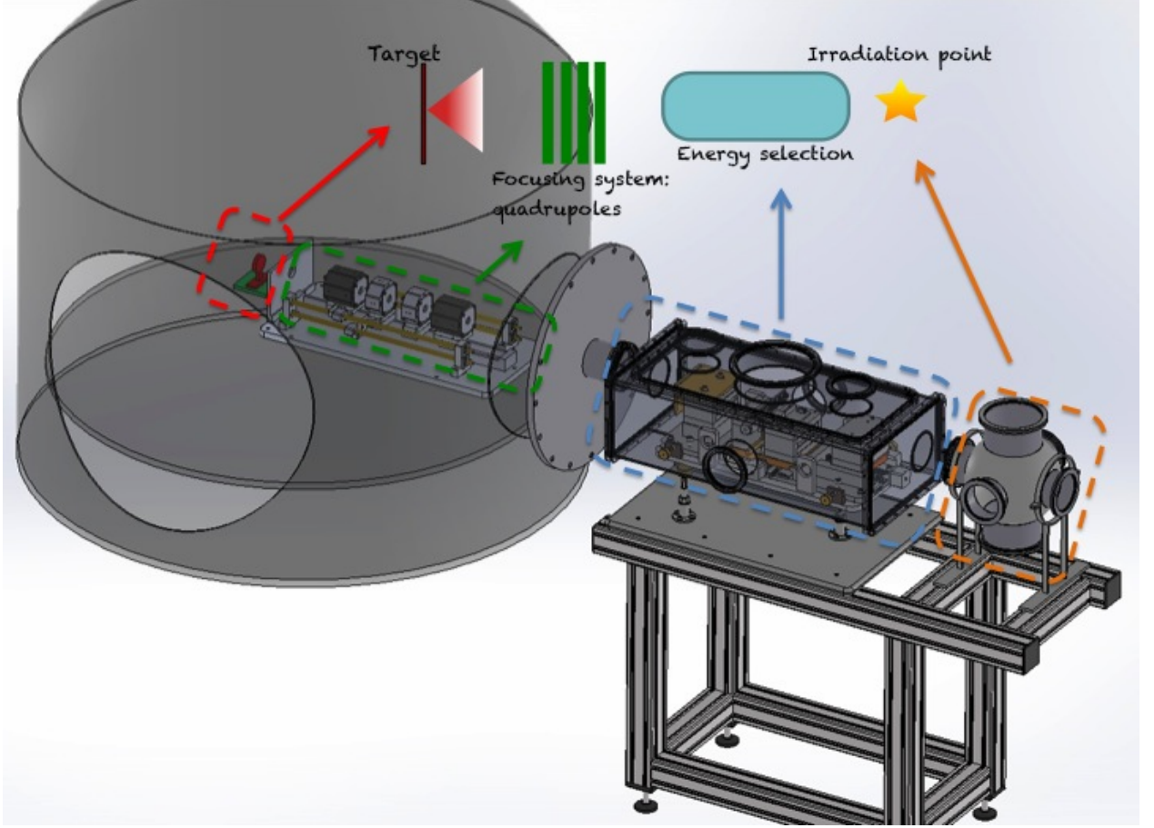
FIGURE 4.3: Draft of the developed prototypes assembled in a possible proposed configuration. On the basis of these prototypes the final elements of the ELIMAIA beamline is being realised, maintaining some of the developed ideas.
