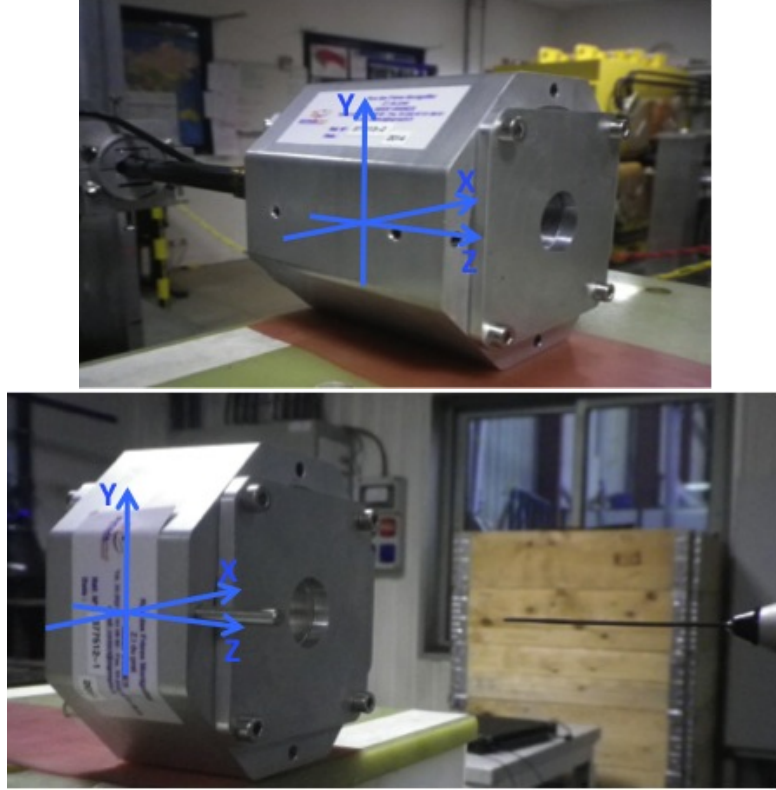
FIGURE 4.6: Long (80 mm ) and short (40 mm) quadrupoles.
