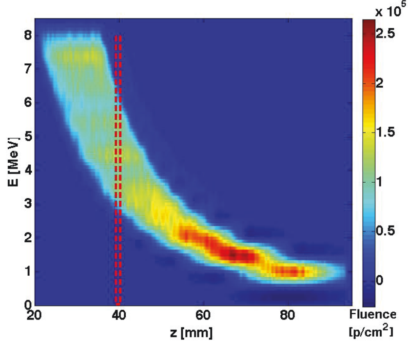
FIGURE 5.13: Protons energy ( E[\text{MeV}] ) vs radial position ( z[\text{mm}] ) on the slit plane, with the fluence distribution described by the colour index. The red dashed lines centered in z = 39.0 mm represents the slit aperture, placed in order to select 4.5 MeV.
