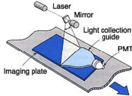
FIGURE A.4: Principle of reading the radiation image from the Imaging Plate: the exposed IP, while being conveyed, is scanned with a focused laser beam. The PSL released upon the laser is collected into the photomultiplier tube (PMT) through the light collection guide and is converted to electric signals.
