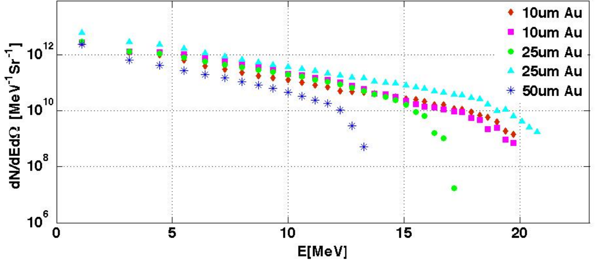
FIGURE 3.8: Energetic distributions of the proton beams generated from the laser interaction with 10, 25 and 50 \mu\text{m} thick, Au targets.
