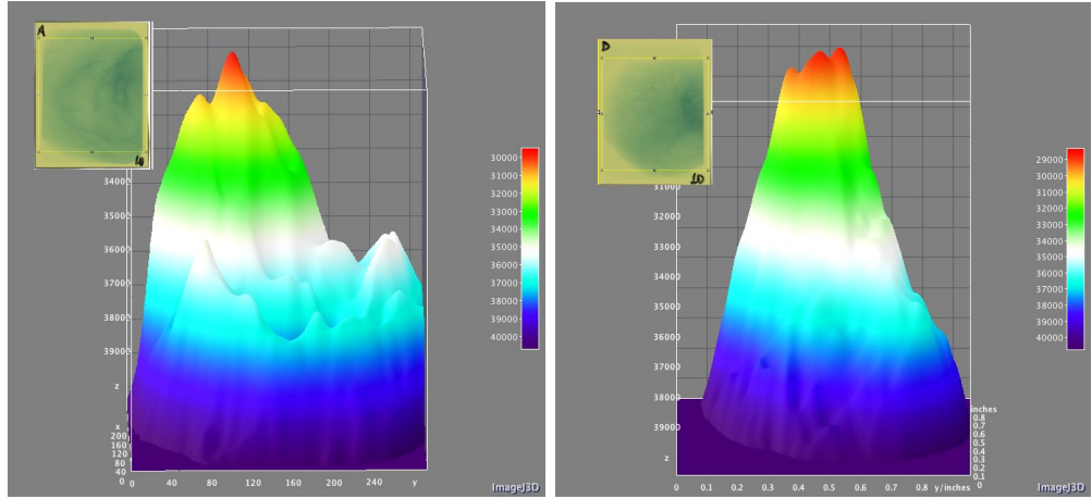
FIGURE 3.9: 3D beam profiles of the selected ROIs (yellow rectangle) in the 10th films of the stacks irradiated using the 10 \mu\text{m} (left) and 25 \mu\text{m} (right) thick targets. This plot are obtained using ImageJ.
