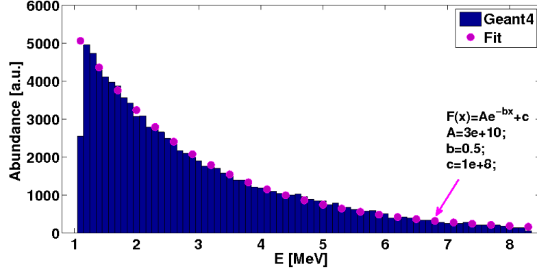
FIGURE 6.3: Typical laser-driven proton spectrum, used as simulation input.
