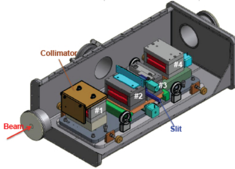
FIGURE 4.11: AutoCad scheme of the Energy Selector system in its dedicated chamber.
