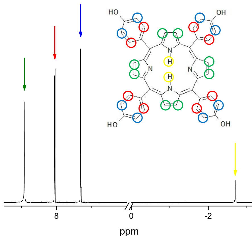
Figure 3.1.5: ^1\text{H} -NMR spectrum of \text{H}_2\text{TPP} in acetone- \text{d}_6 .
