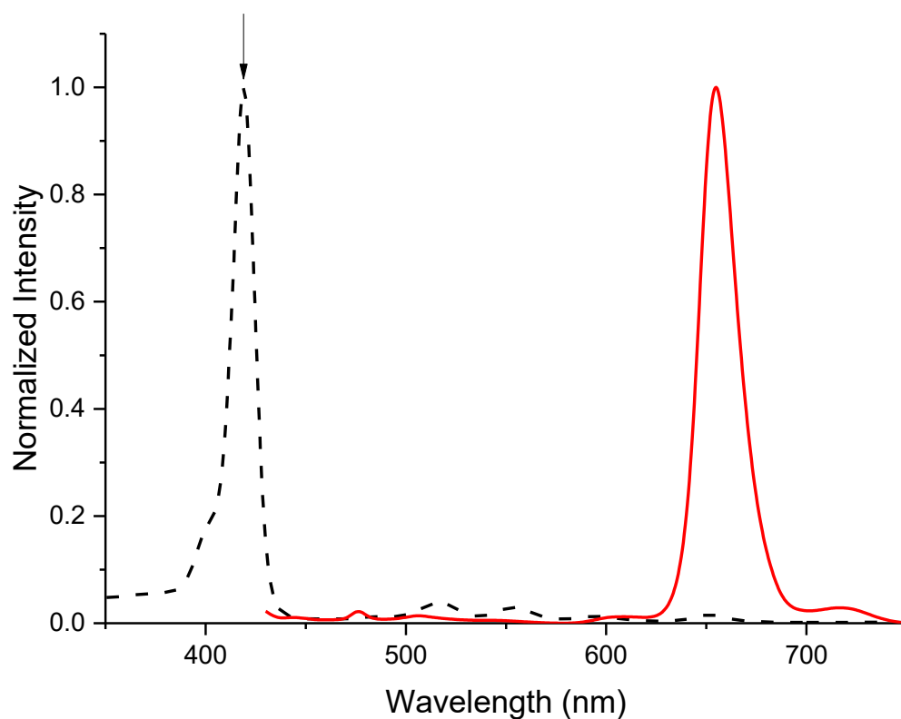
Figure 3.1.7: In red, the fluorescence spectrum of a solution of \text{P(OH)}_4 ( c = 1 \times 10^{-6} \text{ M} ) in acetone. In black, the Uv-Vis spectrum of the same solution. The arrow indicates the wavelength at which the sample is excited (419 nm, maximum Soret Band) to obtain the fluorescence spectrum.
