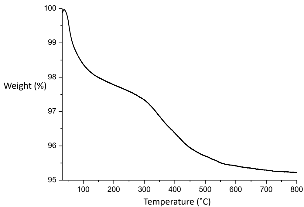
Figure 3.5.7: TGA analysis in \text{N}_2 of \text{Fe}_3\text{O}_4 nanoparticles after treatment at 500 ^{\circ}\text{C}
