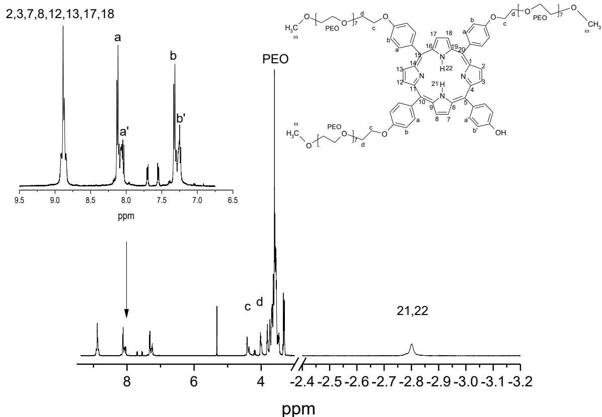
Figure 3.2.5: ^1\text{H} -NMR spectrum in \text{CD}_2\text{Cl}_2 of \text{P}(\text{PEG350})_3
