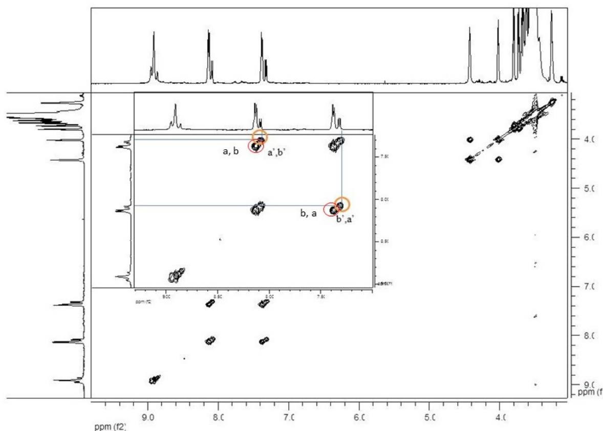
Figure 3.2.14: ^1\text{H} - ^1\text{H} -COSY spectrum of P (PEG750) _3 in acetone- \text{d}_6 . The inset shows the magnification of the signals in the range of 7-9ppm and the related correlations.
