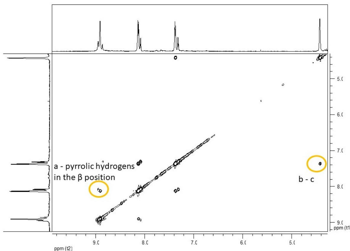
Figure 3.2.13: ^1\text{H} - ^1\text{H} -ROESY spectrum of P (PEG750) 3 in acetone- \text{d}_6 .
