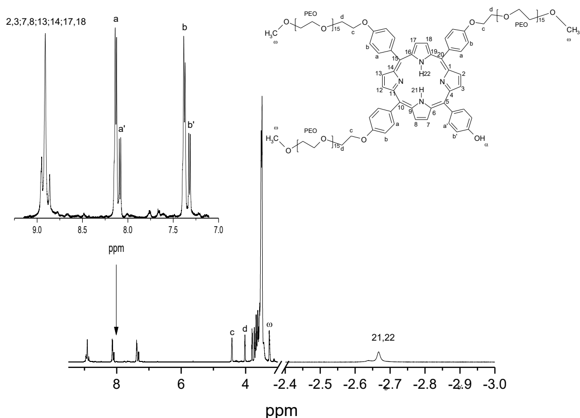
Figure 3.2.12: ^1\text{H} -NMR spectrum of \text{P}(\text{PEG } 750)_3 . The spectrum was acquired using acetone- \text{d}_6 as solvent.
