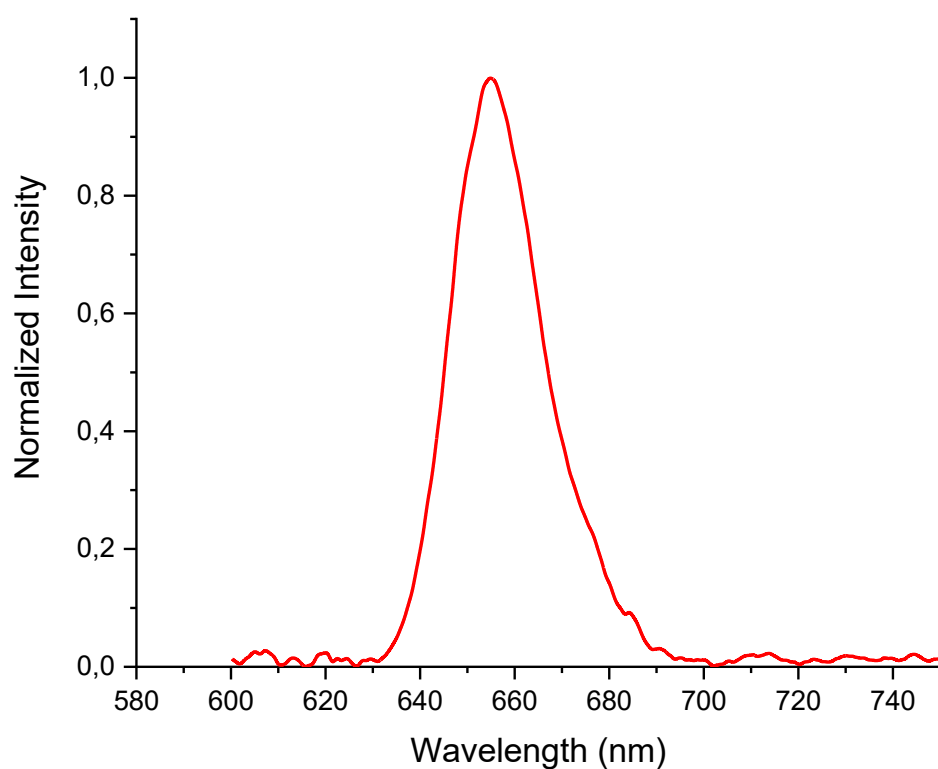
Figure 3.4.23: Fluorescence spectrum of AuNPs functionalized with 3-chloro-propanediol and P(PEG750) 3 ( \lambda_{\text{exc}} =423 nm). The spectrum was acquired using a 405 nm filter in front of the detector.
