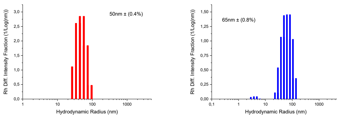
Figure 4.1.22: In red, the size distribution of AuNPs@P(PEG350) 3 nanoparticle in acetone. In blue, the size distribution of AuNPs@P(PEG350) 3 nanoparticle in water.
