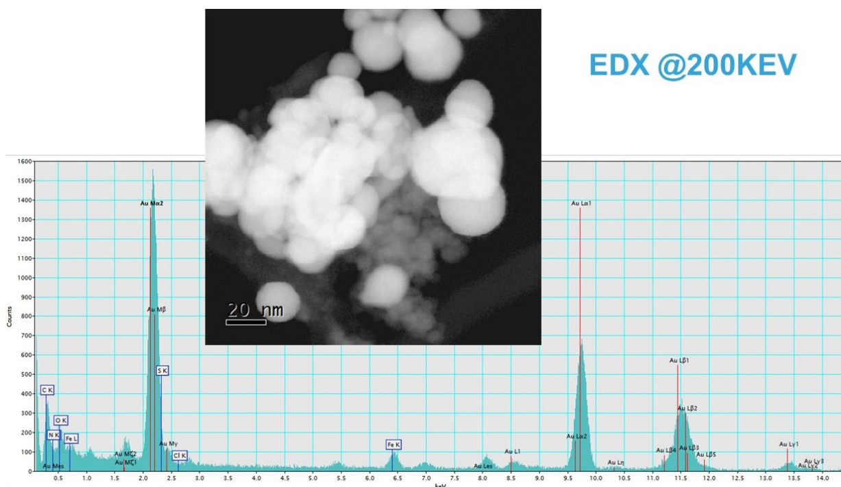
Figure 4.1.30: EDX analysis of \text{Fe}_2\text{O}_3@\text{Au}@\text{P}(\text{PEG}350)_3 nanoparticles.
