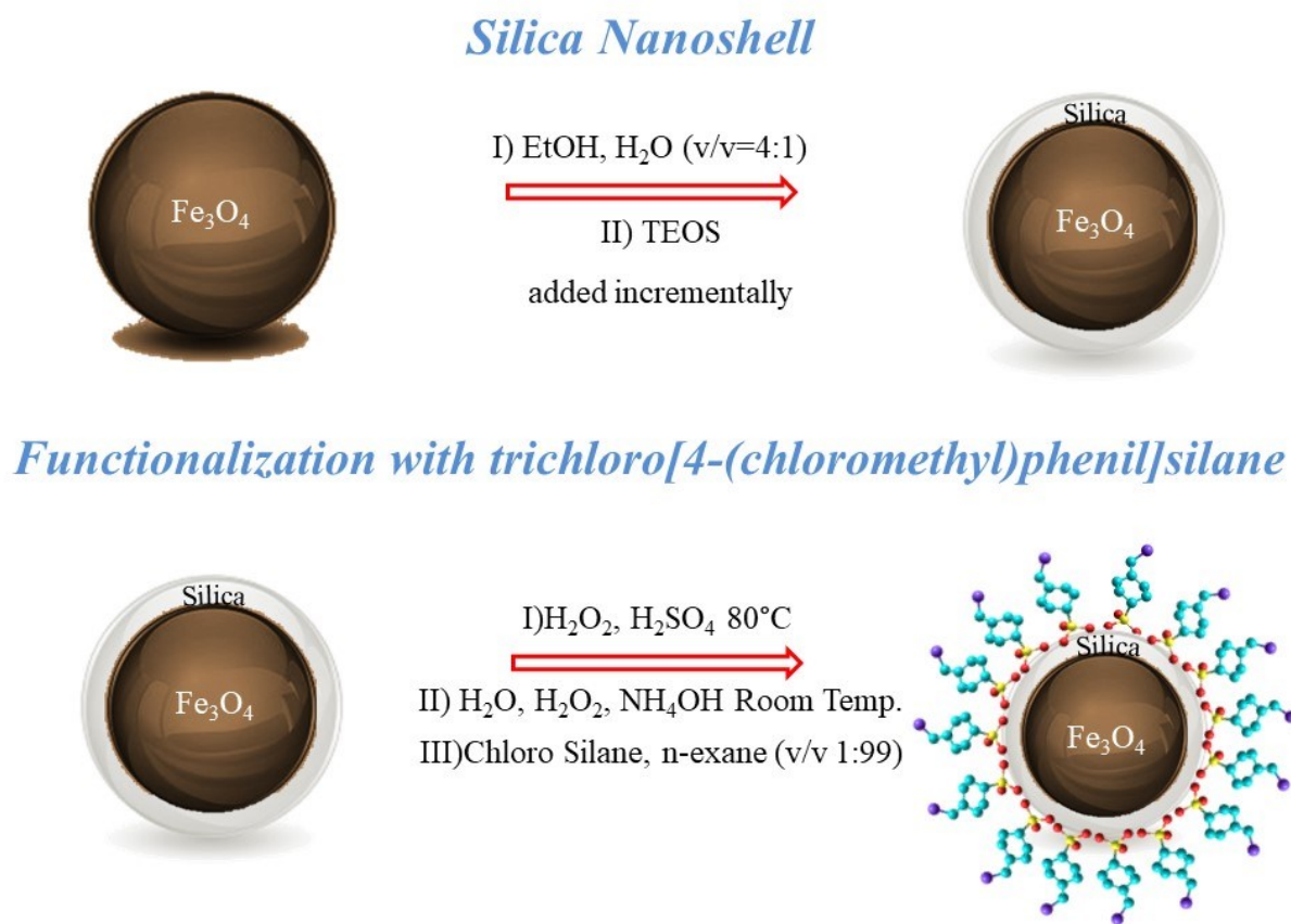
Figure 3.6.1: Synthesis of silica nanoshell on \text{Fe}_3\text{O}_4 nanoparticles, and functionalization with trichloro[4-(chloromethyl)phenyl]silane.
