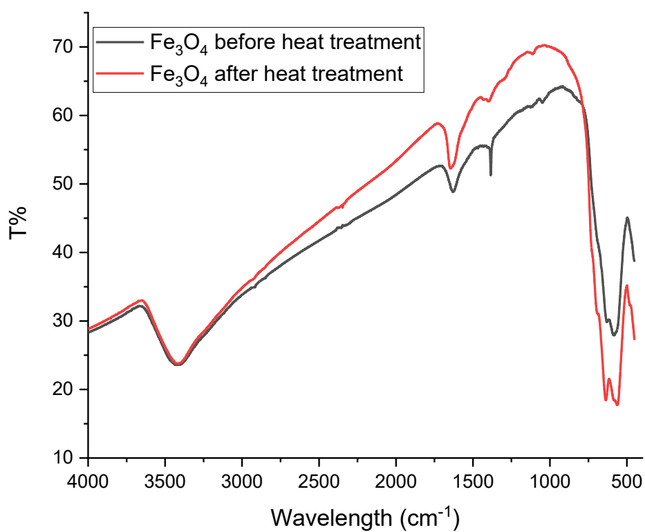
Figure 3.5.6: IR spectra of the nanoparticles of \text{Fe}_3\text{O}_4 nanoparticles before heat treatment (black) and after heat treatment (red).
