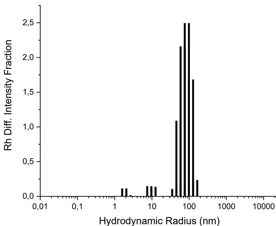
Figure 3.6.3: Size distribution of \text{Fe}_3\text{O}_4@\text{SiO}_2 Nanoparticles in water solution
