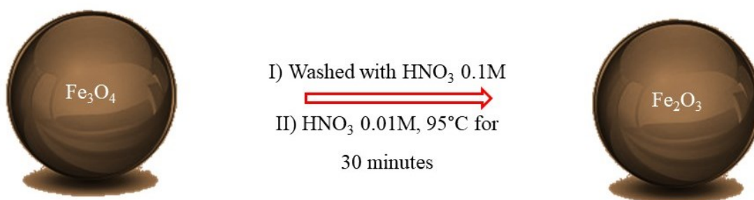
Figure 3.7.1: Synthesis scheme of Fe 2 O 3 nanoparticles.
