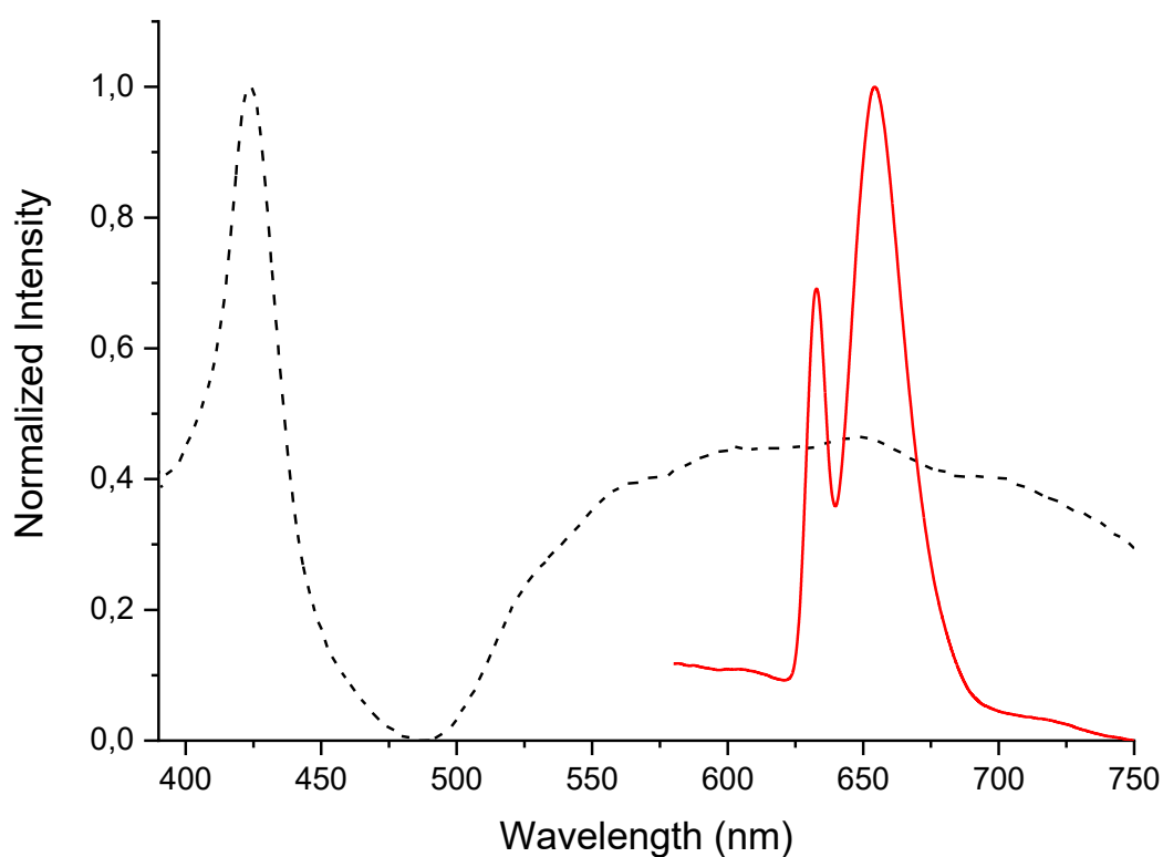
Figure 3.4.22: In black, UV-Vis spectrum of AuNPs functionalized with 3-chloro-propanediol and P(PEG750) 3 in water; in red, the corresponding fluorescence spectrum of the same solution ( \lambda_{\text{exc}}=423 nm).
