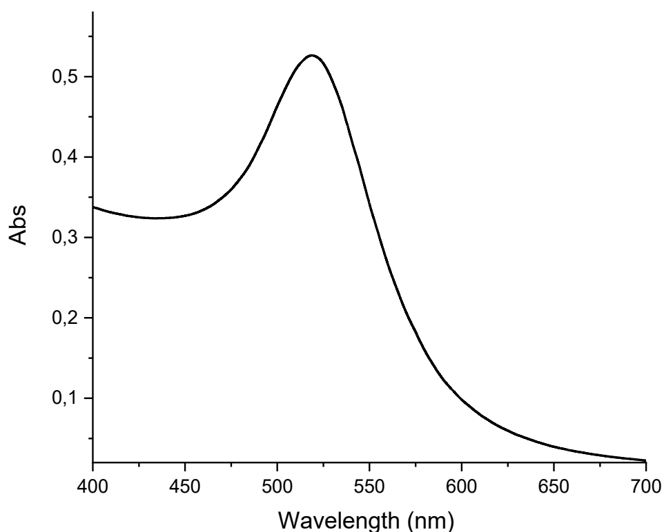
Figure 3.4.4: Uv-Vis spectrum of AuNPs in aqueous solution.
