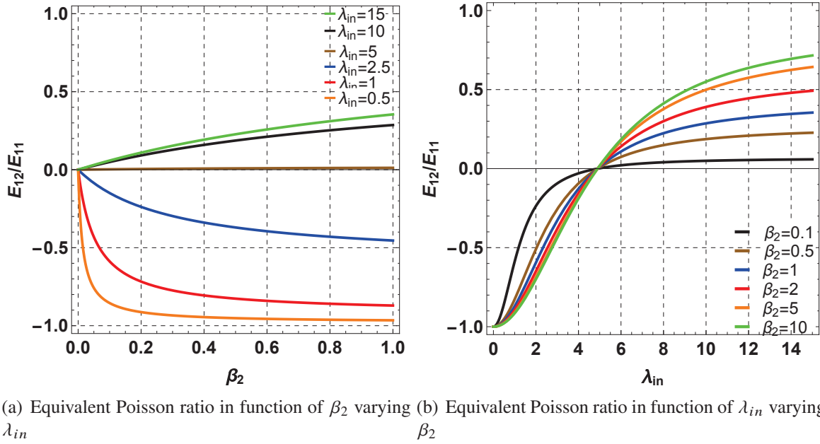
Figure 3.19: Equivalent Poisson ratio in the case of material with reference cell square braced with rigid connections
