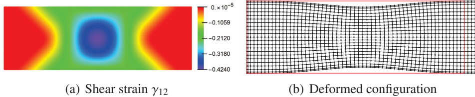
Figure 4.21: Shear strain \gamma_{12} and deformed configuration, with the shear modulus G_{12} = 0 , obtained via isogeometric analysis - Aspect ratio of the specimen 3:1
