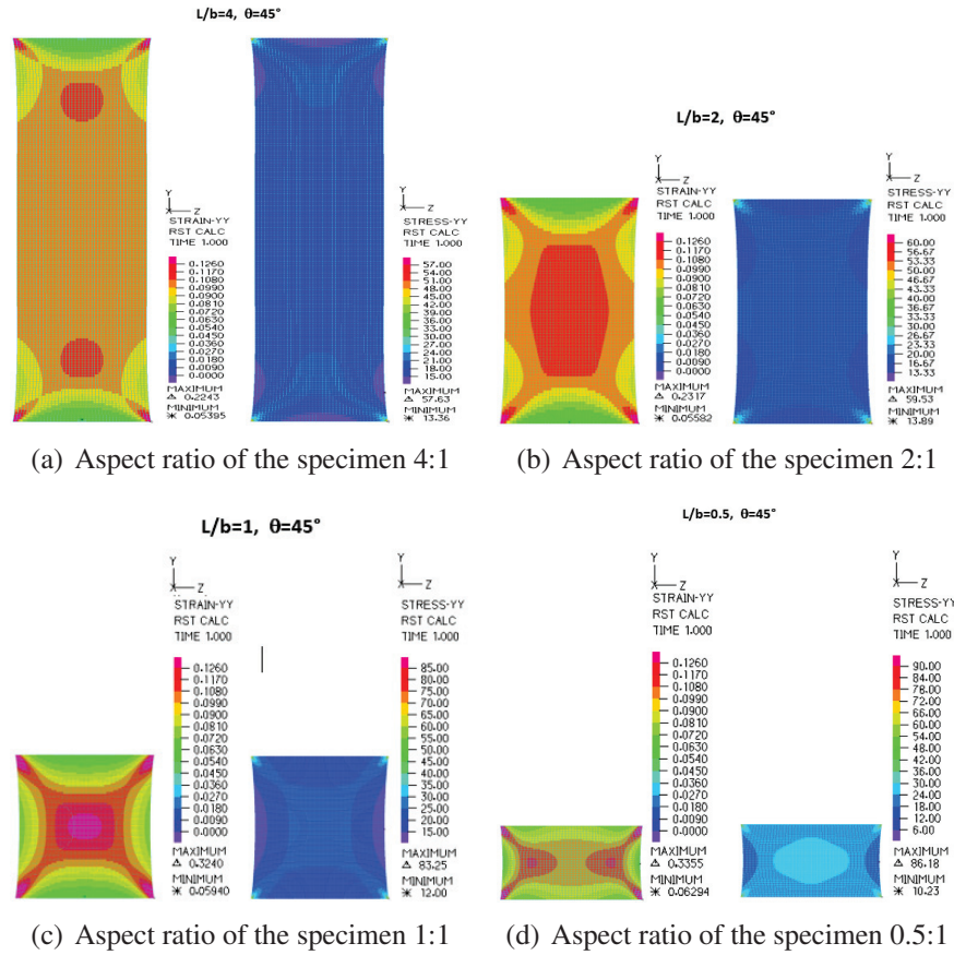
Figure 4.4: Plot of the strain \varepsilon_{yy} and the stress \sigma_{yy} for bias test of a network with square braced cell with rigid connections. Ratio of the Young modulus of the internal fibres to the Young modulus of the mean fibres, equal to 1/5.
