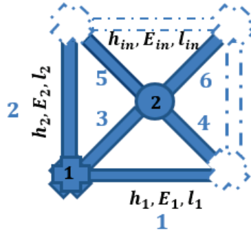
Figure 3.16: Braced cell
