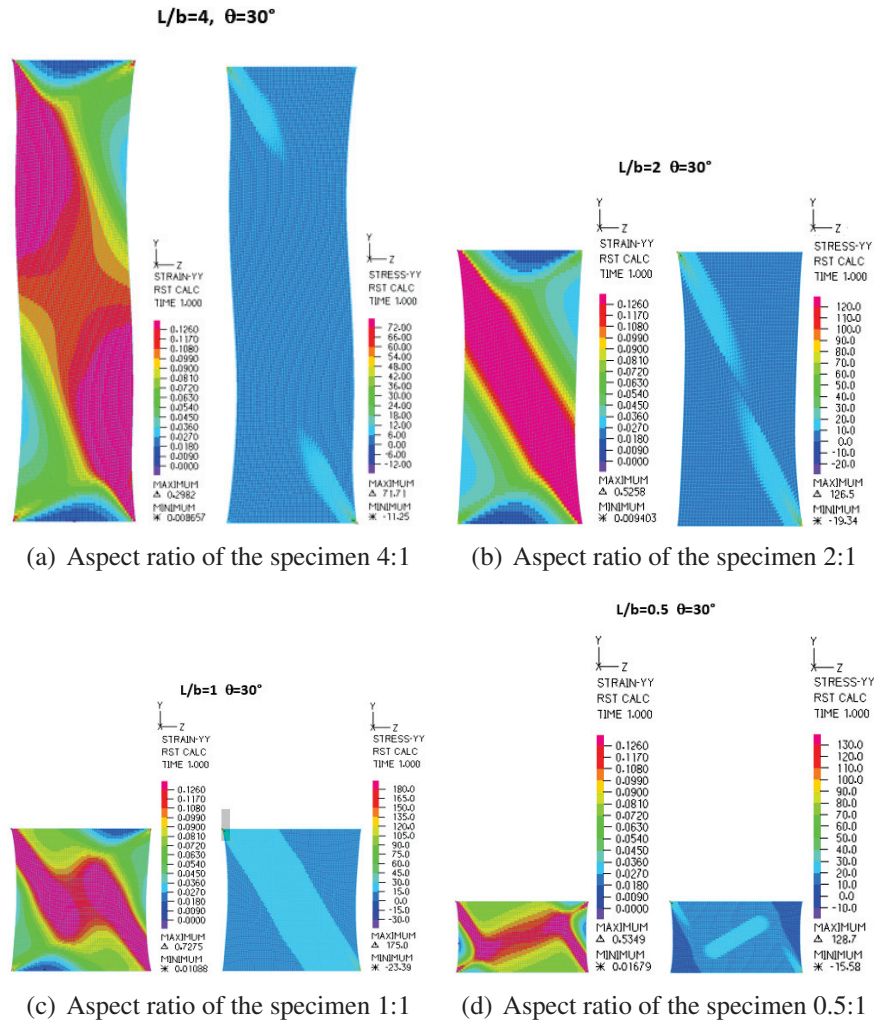
Figure 4.8: Plot of the strain \varepsilon_{yy} and the stress \sigma_{yy} for an extension test of a network with square reference cell having the fibre's direction rotated by \theta = 30^\circ respect the axis of the specimen.
