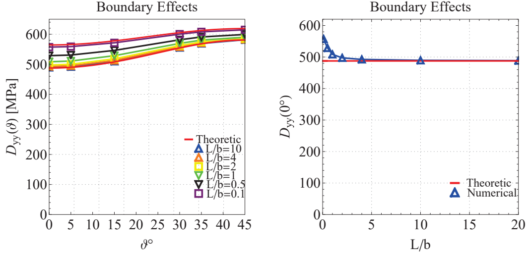
(a) Apparent elastic modulus of the specimen D_{yy} as function of the fibre direction for different aspect ratio of the specimen (b) Apparent elastic modulus D_{yy} as function of different aspect ratio of the specimen for the main fibre direction rotated by 0^\circ respect the specimen axis.
