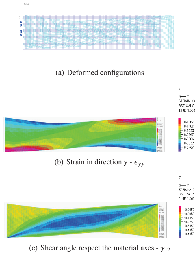
Figure 4.17: Extension test in network material with skew cell - angle between the fibres is equal to \alpha = 30
