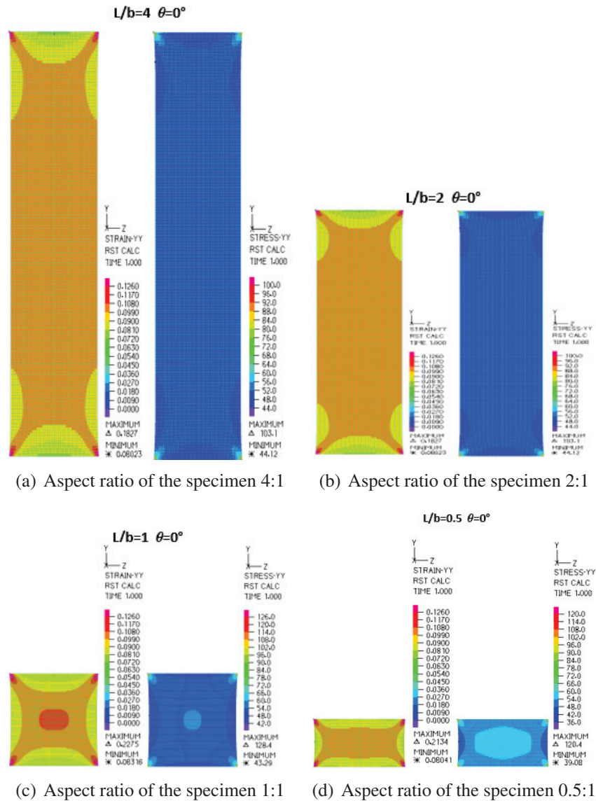
Figure 4.10: Plot of the strain \epsilon_{yy} and the stress \sigma_{yy} for an extension test of a network with square braced cells rigidly connected having the main fibre's direction coincident to the axis of the specimen.
