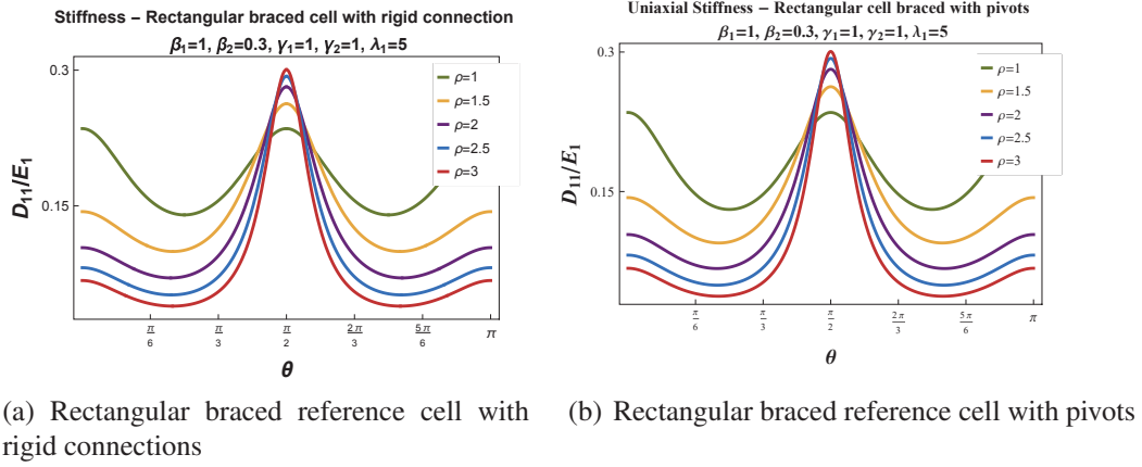
Figure 3.23: Uniaxial stiffness D_{11} as function of the angle \theta with \beta_2 = 0.3 and varying the aspect ratio \rho .
