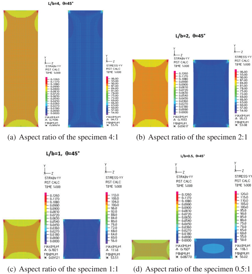
Figure 4.5: Plot of the strain \varepsilon_{yy} and the stress \sigma_{yy} for bias test of a network with braced cell connected by pivots varying the aspect ratio of the specimen.
