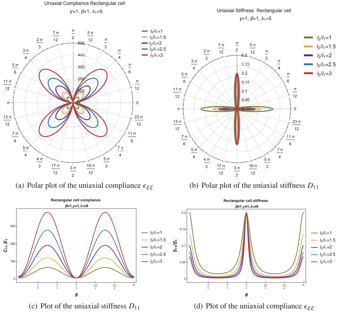
Figure 3.13: Uniaxial compliance and stiffness of a material formed by rectangular reference cell with rigid connection as function of the load directions for different aspect ratio of the length
