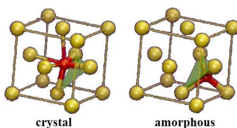
Figure 2.10 Local structure of a Ge:Sb:Te systems around Ge atoms in the crystalline and in the amorphous phase, according to the umbrella-flip model. Stronger bond are shown thicker than weaker bonds. Coordination changes from tetrahedral to octahedral upon crystallization [Kol04].
