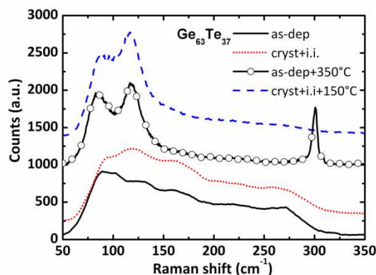
Figure 4.17 Raman spectra of different Ge-rich samples: as deposited (solid line), ion amorphized with 10^{14} \text{ Ge}^+ ions (red dotted line), ion amorphized and annealed at 150^\circ\text{C} (blue dashed line), as deposited and annealed at 350^\circ\text{C} (circles and solid line).
