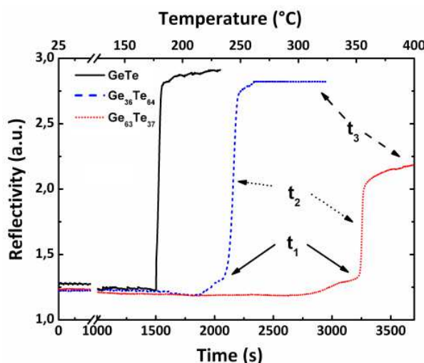
Figure 4.7 Time resolved reflectivity measurements, during an heating ramp of 6^\circ \text{C/min} , of three different \text{Ge}_x\text{Te}_{1-x} alloys ( x=0.36, 0.51, 0.63 ). We prepared three samples, for both the non-stoichiometric composition, by stopping at different times the annealing process. The arrows point to these different times.
