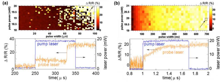
Figure 2.14 (a) \Delta R/R as a function of laser power and duration for a single-pulse experiment on amorphous, as deposited \text{Ge}_4\text{Te}_6 . Arrow points to the laser spot shown in the bottom panel where \Delta R/R is plotted as function of time. (b) The same experiment was also performed on a melt quenched amorphous mark. The crystallization time is smaller [Rao09].
