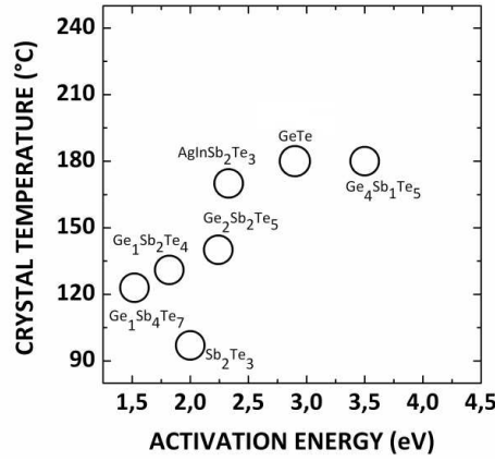
Figure 1.11 Crystallization temperature and activation energy of the crystallization time of several phase change materials. It's clear that the higher is the amount of germanium in the alloy the higher is the crystallization temperature.
