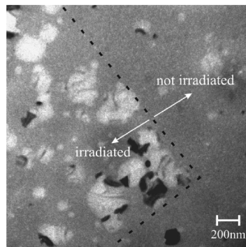
Figure 3.43 TEM plan-view micrographs of as-deposited amorphous GST films implanted with 120 keV 10^{14} Sb + /cm 2 . The presence, during implantation, of a copper mask placed on the sample surface has produced selectively implanted areas next to not implanted areas.
