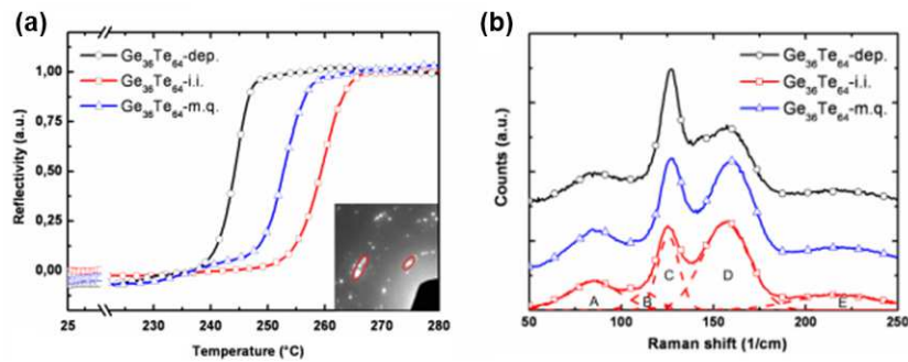
Figure 4.28 (a) Reflectivity vs temperature curves for asdeposited (black), melt quenched (blue), and \text{Ge}^+ irradiated (red) \text{Ge}_{36}\text{Te}_{64} amorphous samples. The inset shows electron diffraction pattern of the annealed sample. The (100) and (110) GeTe spots are circled, whereas the other spots refer to crystalline tellurium. (b) Comparison between the Raman spectra of the three different states of amorphous before the annealing.
