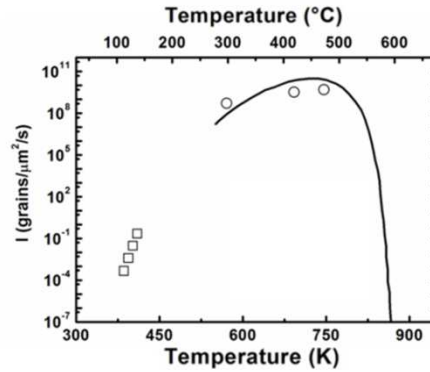
Figure 3.35 Comparison between measured and calculated [Kal05b] nucleation rate as function of temperature.
