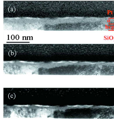
Figure 3.22 TEM cross-sectional images of the hcp GST film implanted by 28 keV \text{Ge}^+ ions at a fluence of 10^{14} ions/cm 2 and annealed in situ at 120 °C for different time until full crystallization. The red lines mark the different layers.
