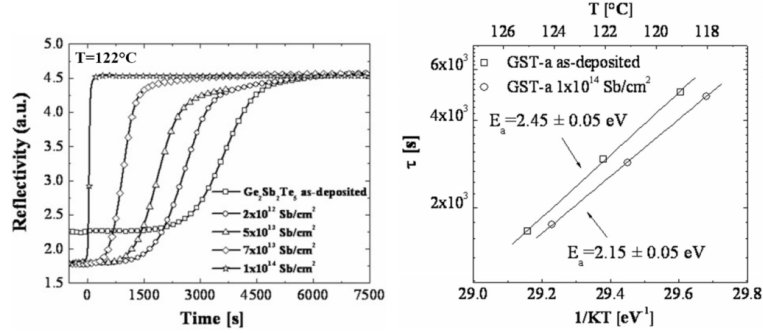
Figure 3.40 (a) Time resolved reflectivity measurements performed on as deposited and ion irradiated GST samples during isothermal annealing at 122°C. (b) Incubation time, as function of 1/k_B T , of as deposited and 10^{14} Sb + /cm 2 ion implanted GST.
