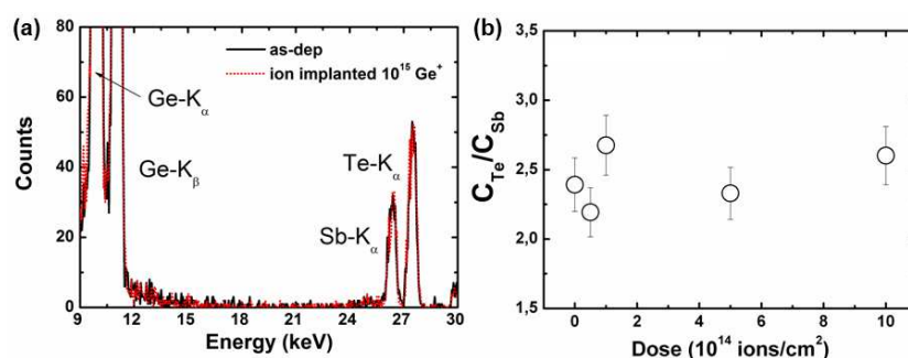
Figure 3.54 (a) PIXE spectra of the as-deposited and Ge + 10 15 ions/cm 2 implanted GST uncapped samples. The He + beam has an initial energy of 2.7 MeV. The K α lines of the different atomic species are clearly reported. (b) The Te/Sb concentration ratio, obtained by the PIXE measurements, is shown as function of the irradiation fluence (uncapped film).
