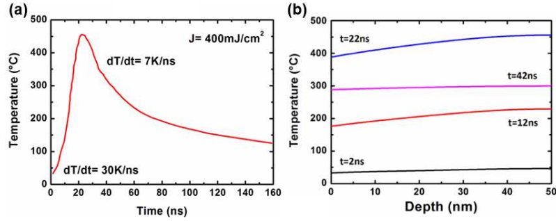
Figure 3.26 (a) Temperature profile as function of time at the the air-GST interface in the case of laser irradiation with a fluence of 400 \text{ mJ/cm}^2 . (b) Corresponding temperature profile inside the GST layer for several times.
