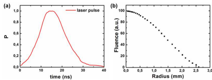
Figure 3.24 Time (a) and spatial (b) energy profile of a single Nd:YAG laser pulse.
