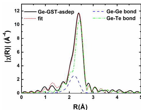
Figure 3.7 The Fourier transform of the k^3\chi plot, reported in fig.3.6, is plotted together with the fit curve (red dotted line) and with the contributions from Ge-Ge (blue dashed line) and Ge-Te bonds (dash-dot green line).
