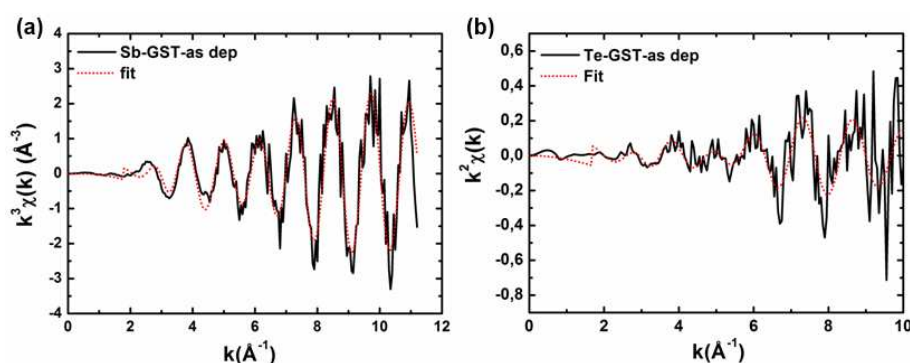
Figure 3.8 The k - \chi plots of the Sb-edge (a) and Te-edge(b) are shown coupled with the corresponding fit curve. The fitting parameters are reported in table 3.1.
