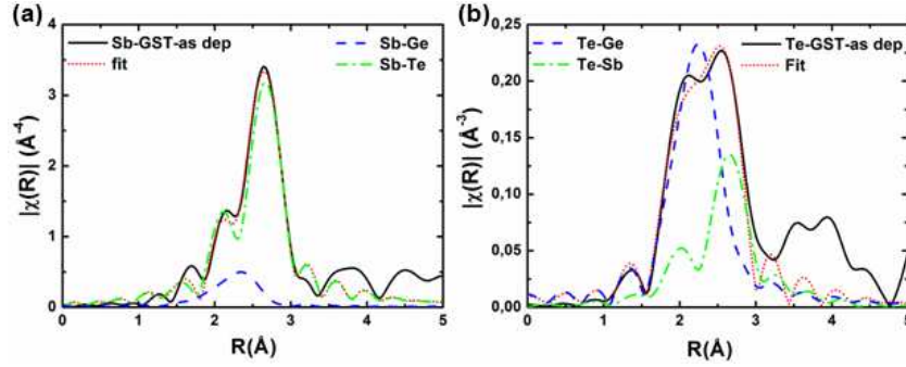
Figure 3.9 The Fourier transform of the k^3\text{-}\chi plot, reported in fig.3.8, are plotted together with the fit curve (red dotted line) and with the contributions from the different bonds.
