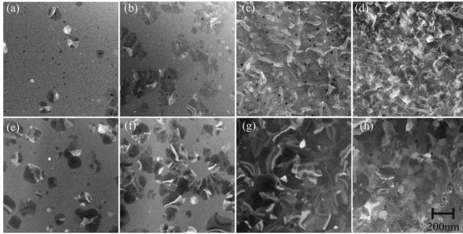
Figure 3.44 STEM plan-view micrographs of as-deposited (top) and ion irradiated (bottom) amorphous GST films, annealed at 122°C with 20% (a)(e), 40% (b)(f), 80% (c)(g), and 100% (d)(h) crystalline fraction. Ion irradiation was performed with 120 keV 10^{14} \text{ Sb}^+/\text{cm}^2 .
