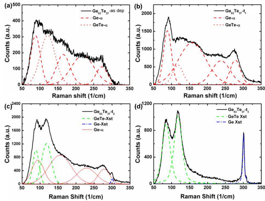
Figure 4.11 (a), (b), (c), (d) Raman spectra of the Ge-rich alloy at different times of the annealing process: as deposited, first stair of the reflectivity curve (time t_1 ), half of the variation of reflectivity (time t_2 ) and complete crystallization (time t_3 ).
